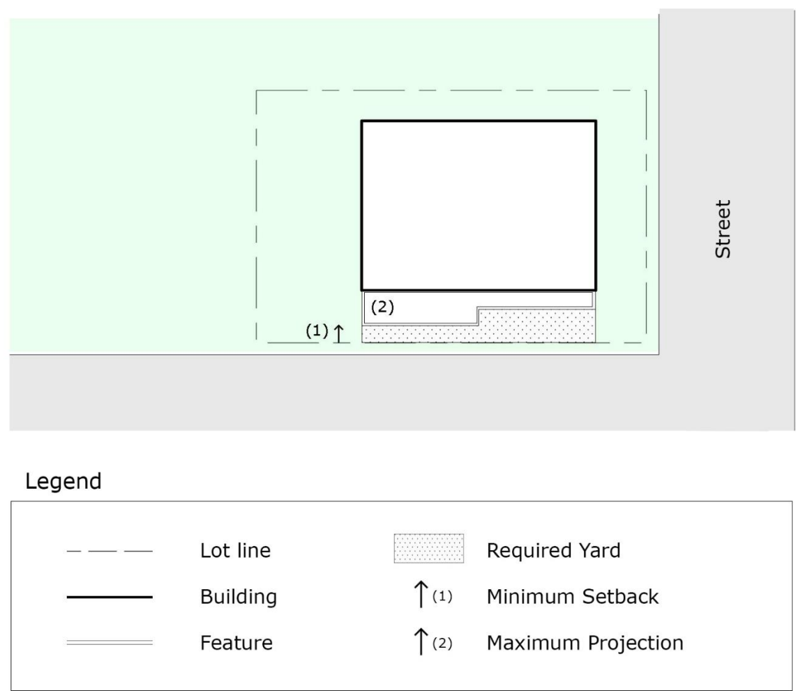
Figure 204-8 demonstrates the minimum setback of one metre and the maximum projection of two metres or 50 per cent of the required yard for a projection not higher than 0.6 metres in a front or exterior side yard.
