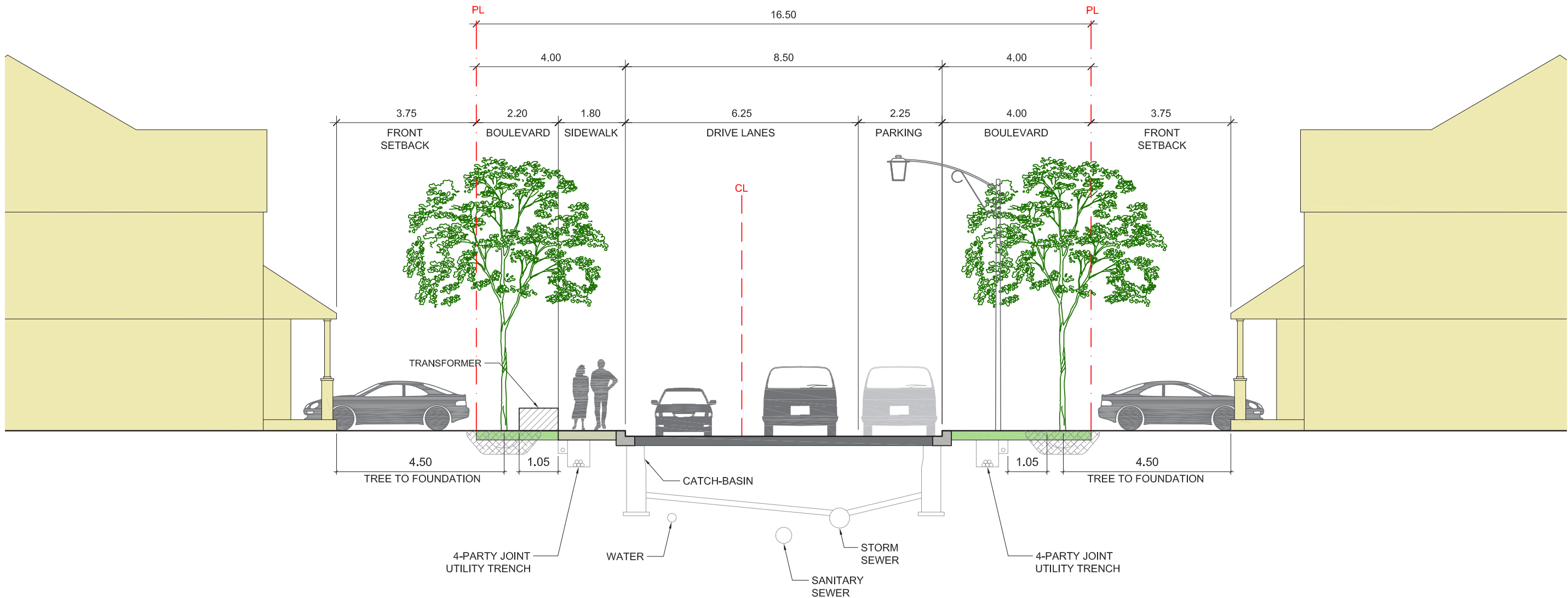
Figure 29 Local Road (Typical 16.5m ROW)
