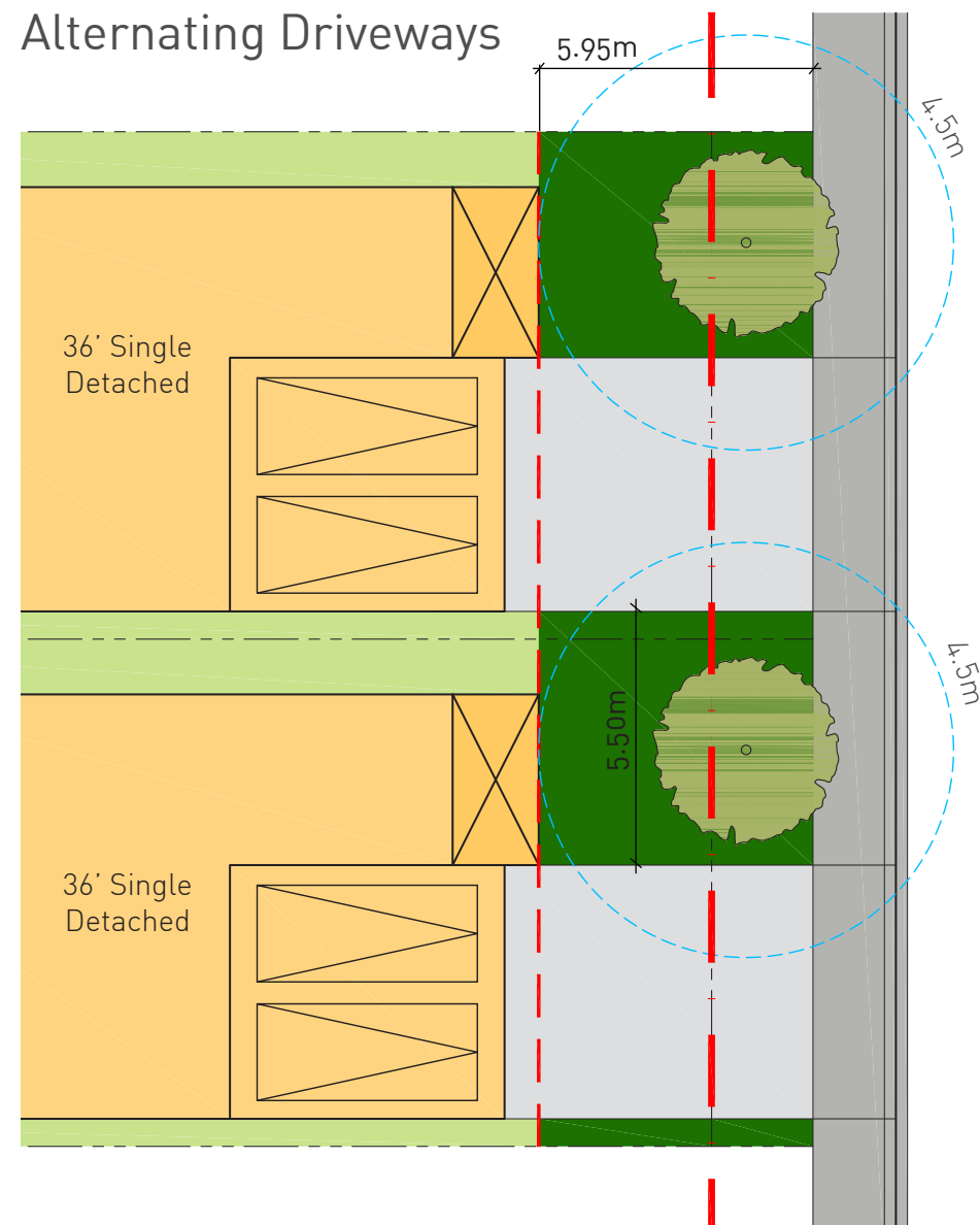
Figure 34 Alternating Driveways
