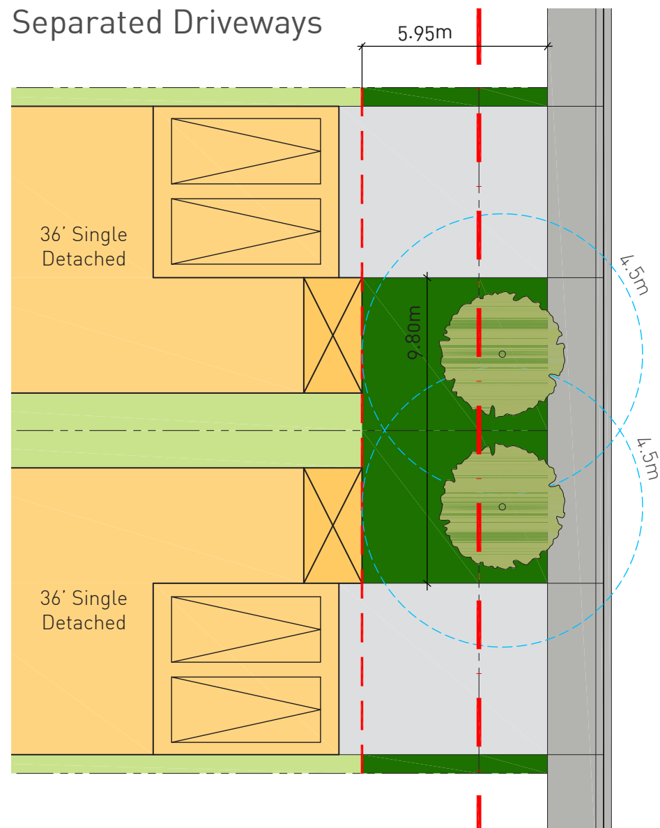
Figure 33 Separated Driveways
