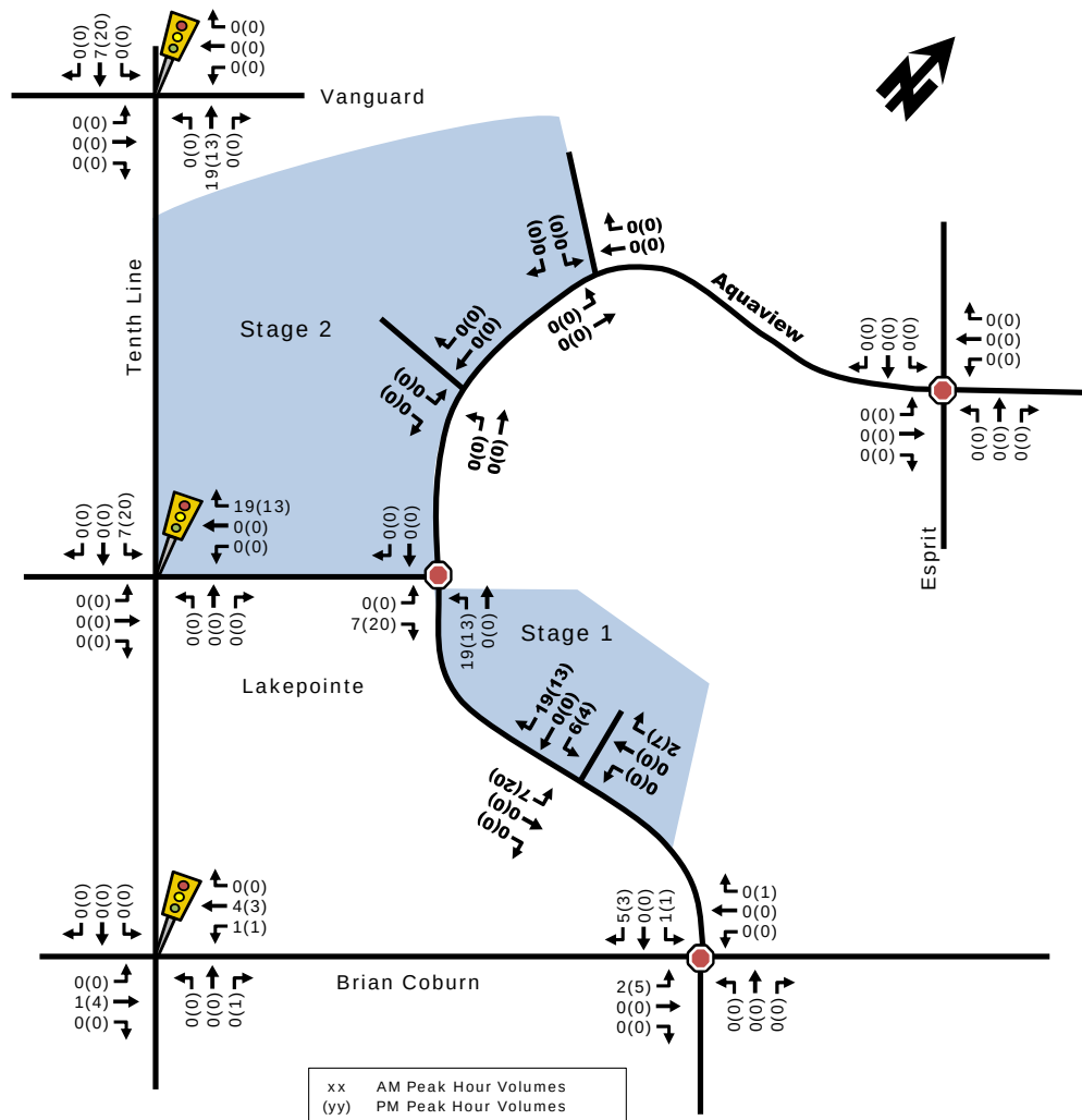
Figure 5: 'New' Stage 1 (Single Homes) Site-Generated Traffic Volumes
