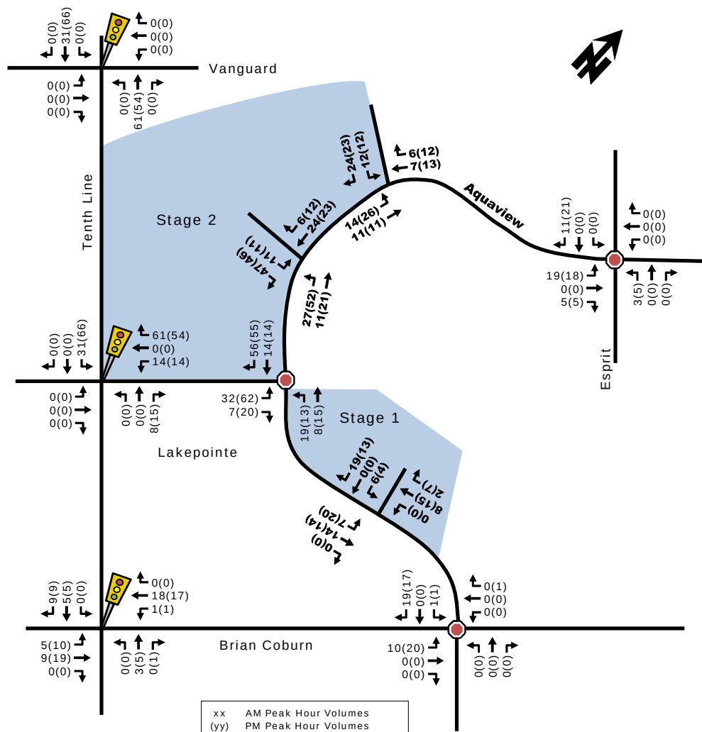
Figure 7: 'New' Total Site-Generated Traffic Volumes
