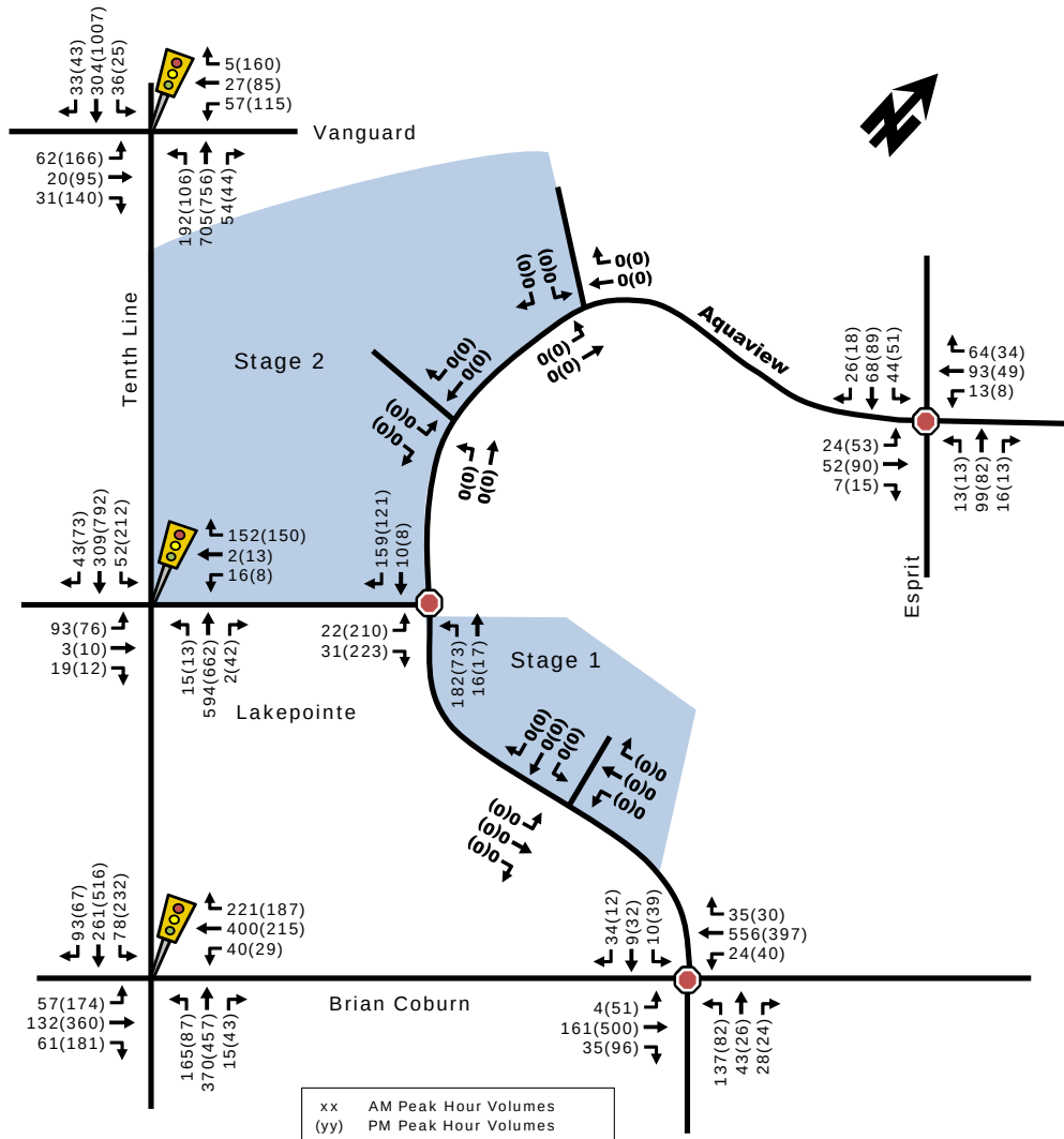
Figure 9: 2025 Background Peak Hour Traffic Volumes
