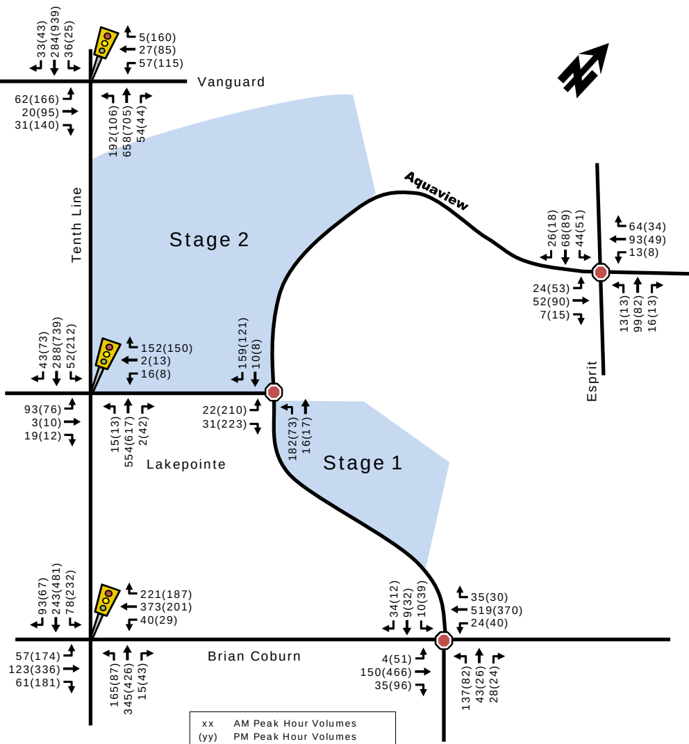
Figure 4: Existing Peak Hour Traffic Volumes
