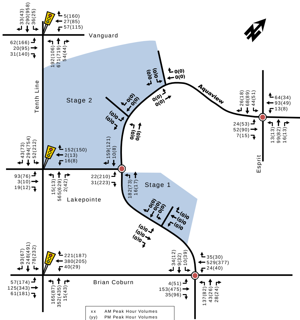
Figure 8: 2020 Background Peak Hour Traffic Volumes
