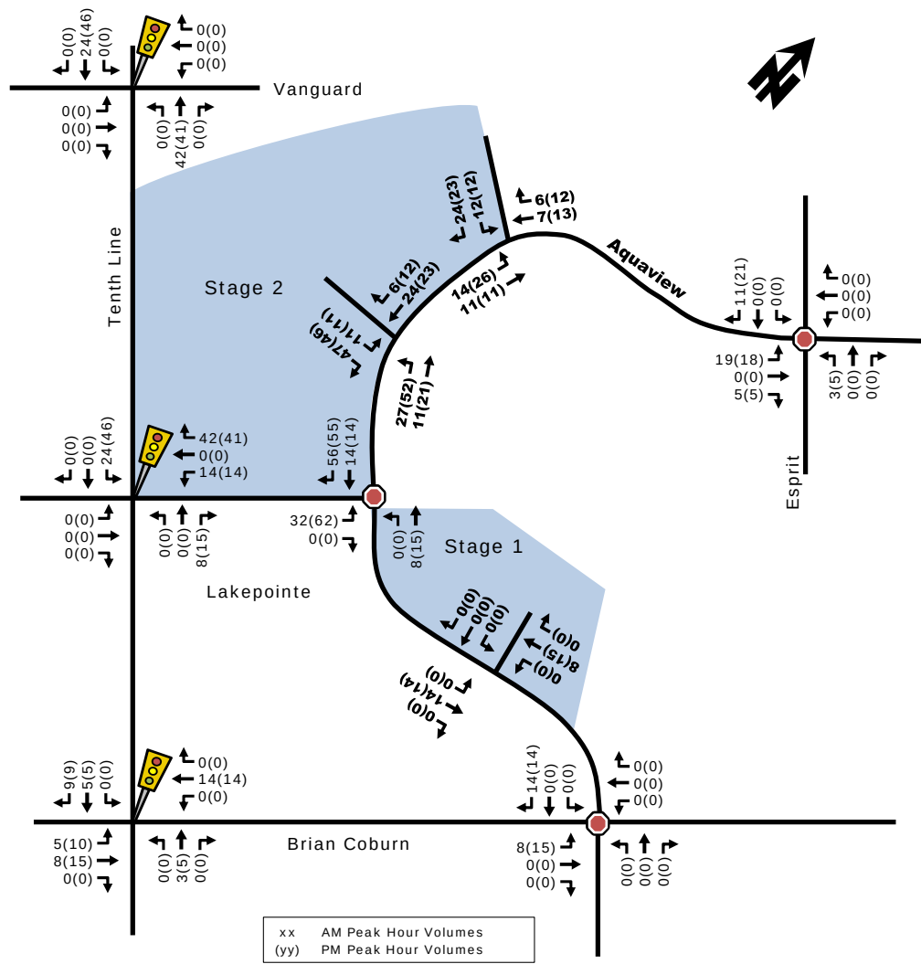
Figure 6: 'New' Stage 2 (Townhomes) Site-Generated Traffic Volumes
