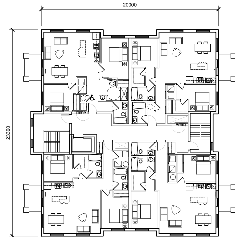
2nd - 4th FLOOR PLAN GFA: 4674 SQ. FT.
