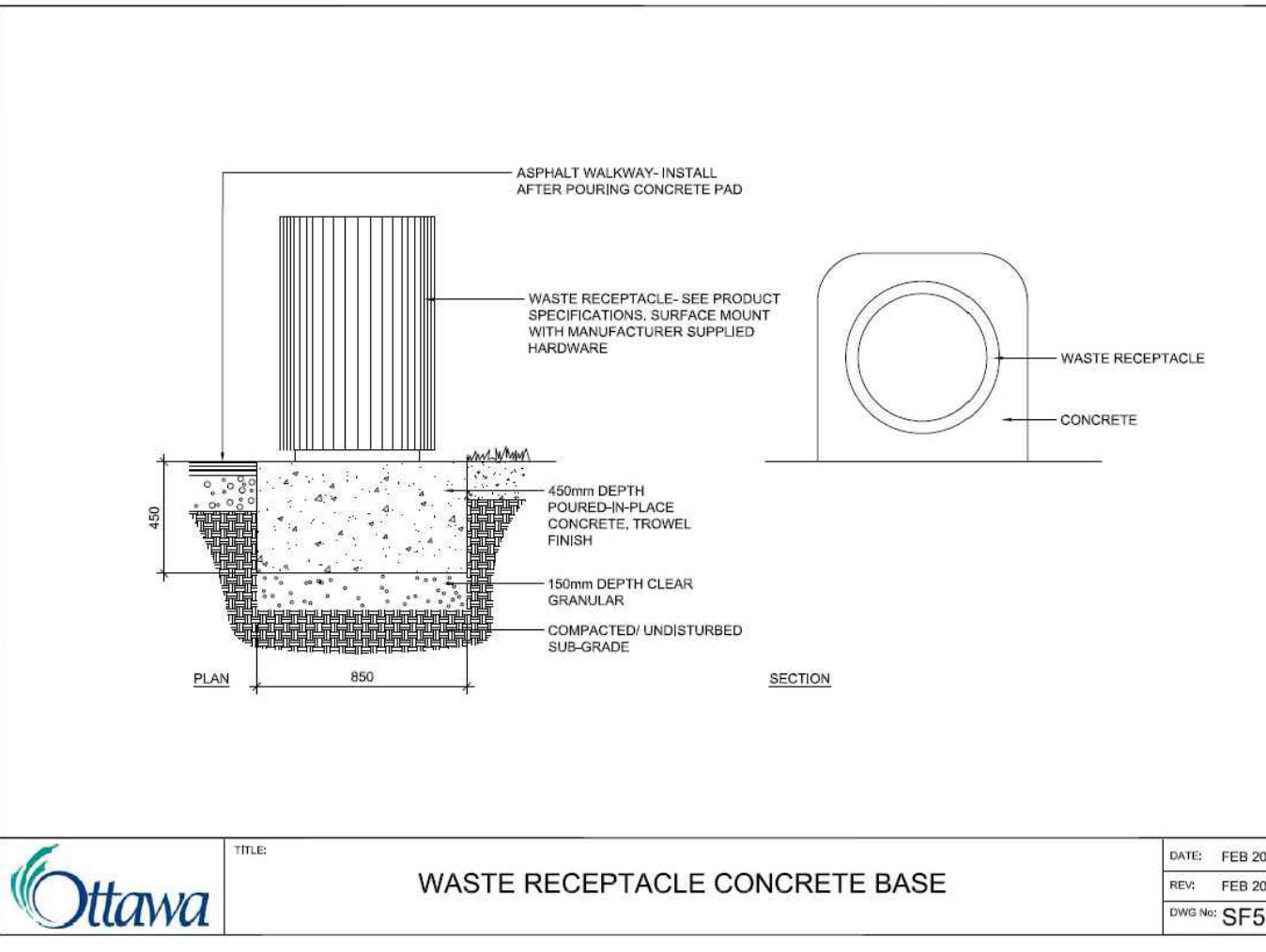
11 WASTE RECEPTACLE MOUNTING ON CONCRETE BASE N.T.S.
