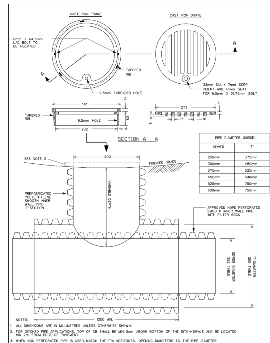
CATCH BASIN - T FOR REAR YARD, DITCHED PIPE AND LANDSCAPING APPLICATIONS
