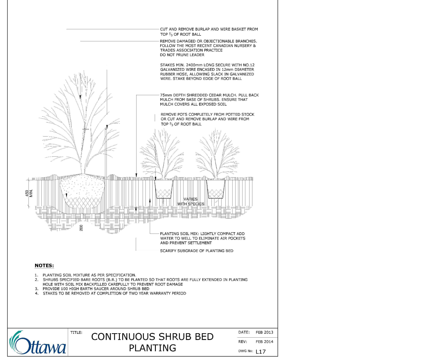
13 CONTINUOUS SHRUB BED PLANTING N.T.S.
