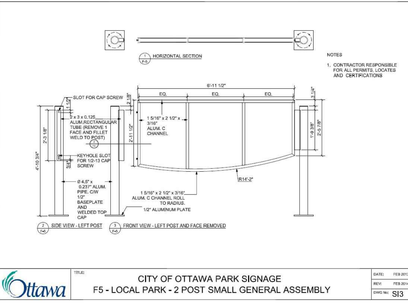
10 LOCAL PARK - 2 POST SMALL GENERAL ASSEMBLY AND INSTALLATION N.T.S.
