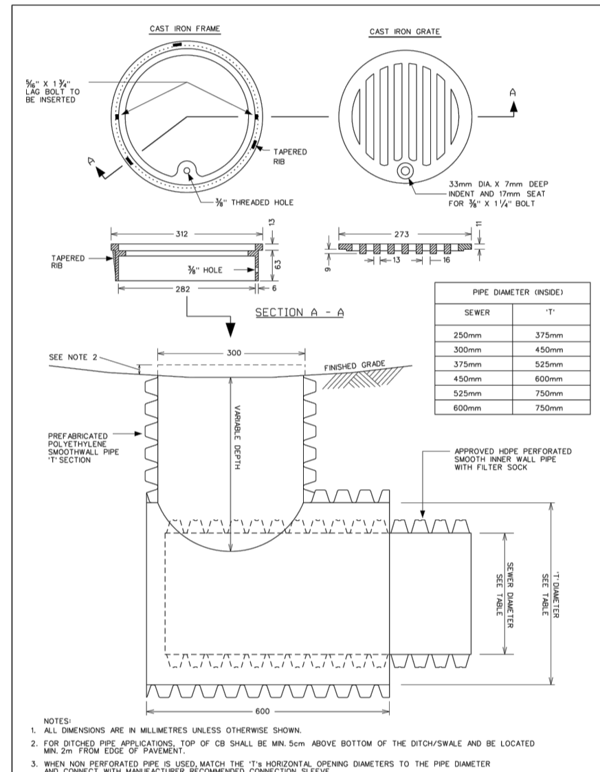
CATCH BASIN - ELBOW FOR REAR YARD, DITCHED PIPE AND LANDSCAPING APPLICATIONS
