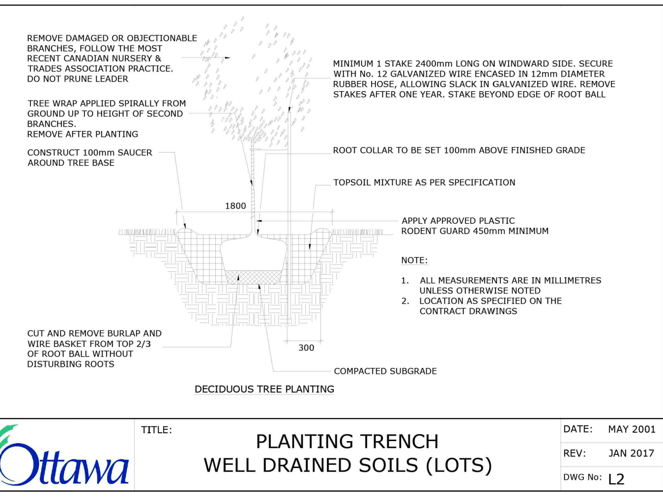
12 DECIDUOUS TREE PLANTING N.T.S.
