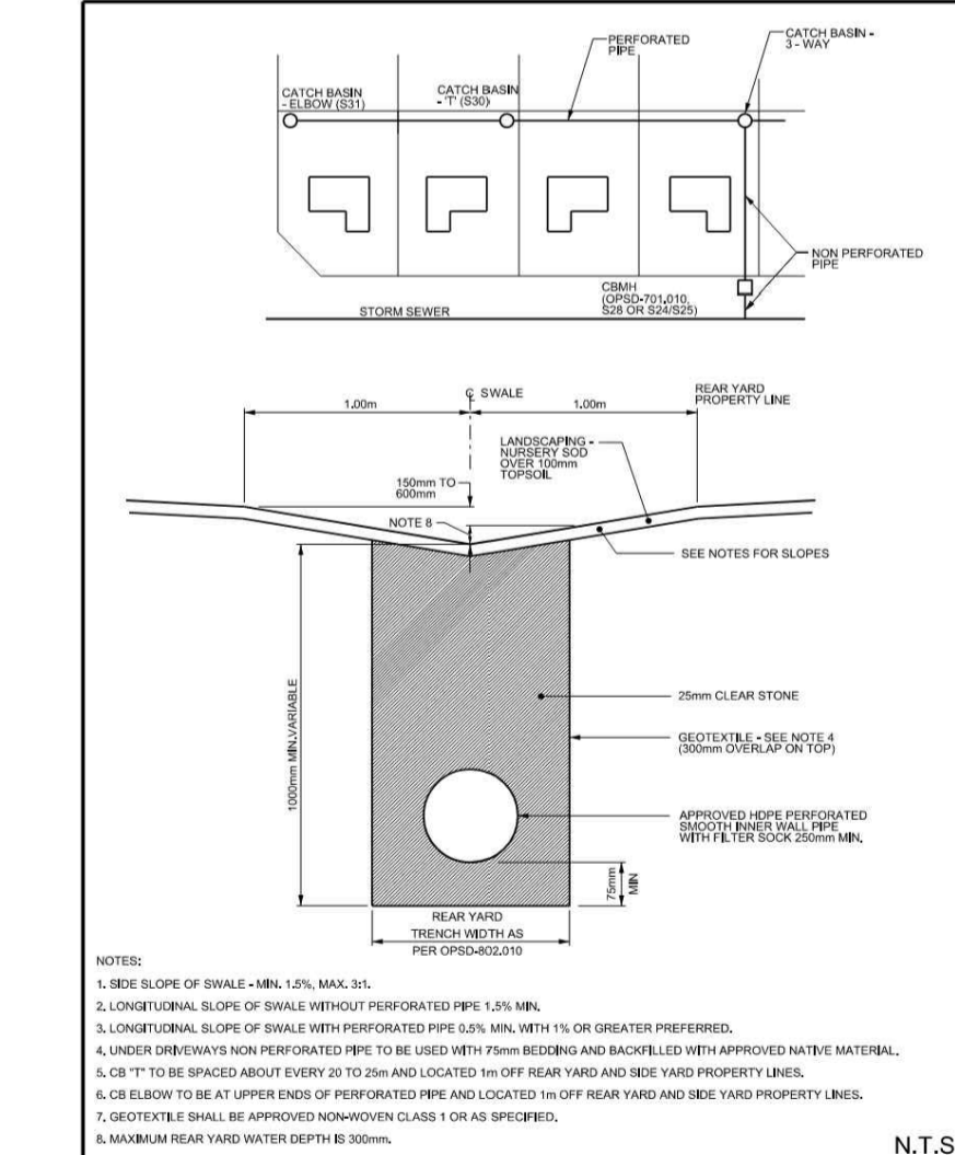
PERFORATED PIPE INSTALLATION FOR REAR YARD AND LANDSCAPING APPLICATIONS
