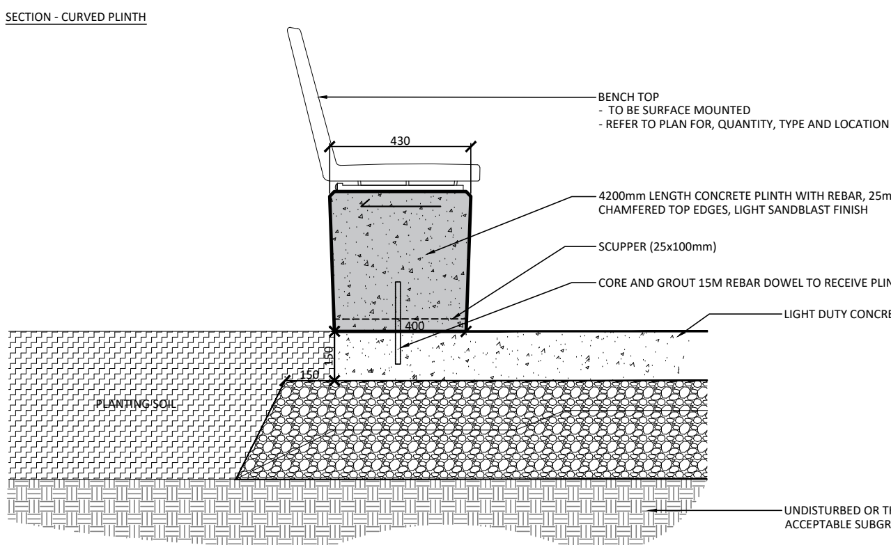
8 PRECAST CONCRETE PLINTHS 1:16
