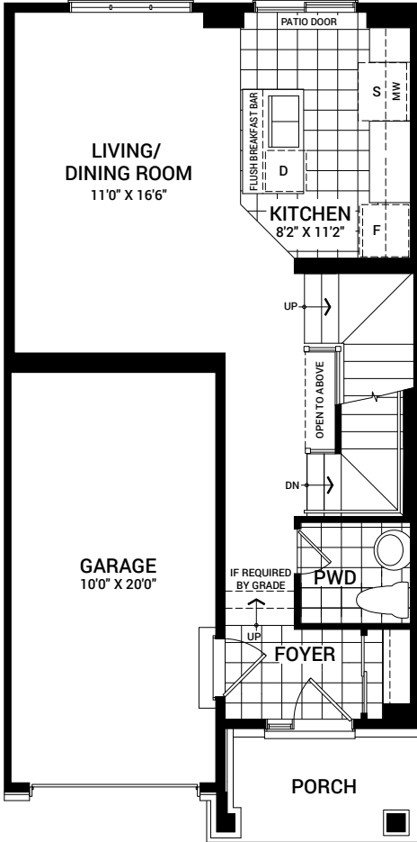
MAIN FLOOR PLAN B
