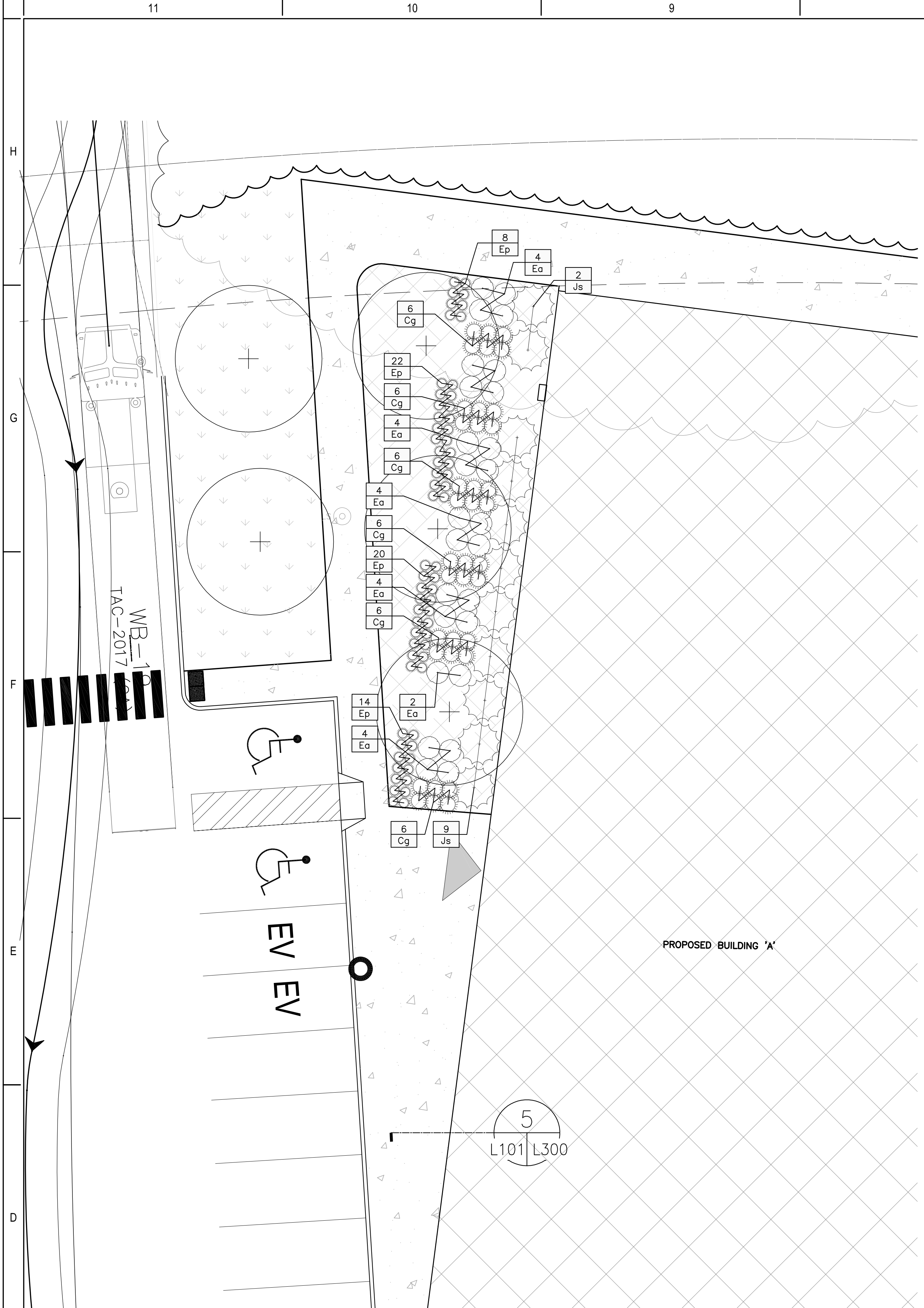
2 PLANTER DETAIL PLAN L101 1:100
