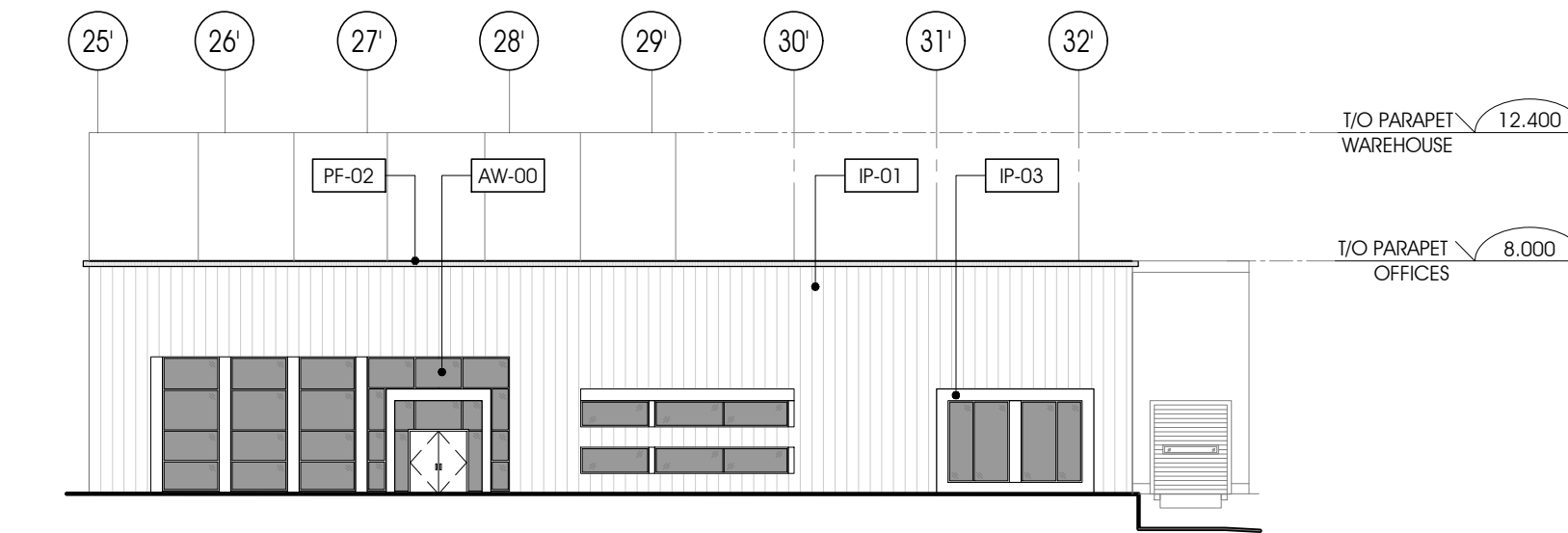
3 OFFICE ELEVATION - HEAD ON A1.1 1:250
