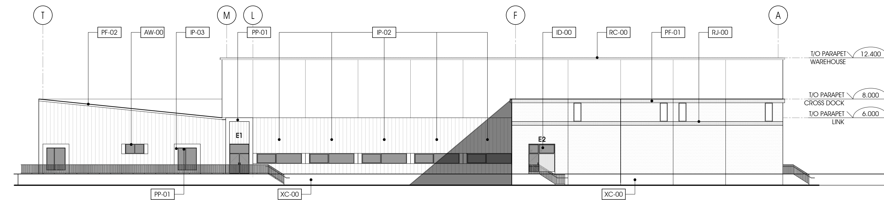
3 EAST ELEVATION A1.1 1:250
