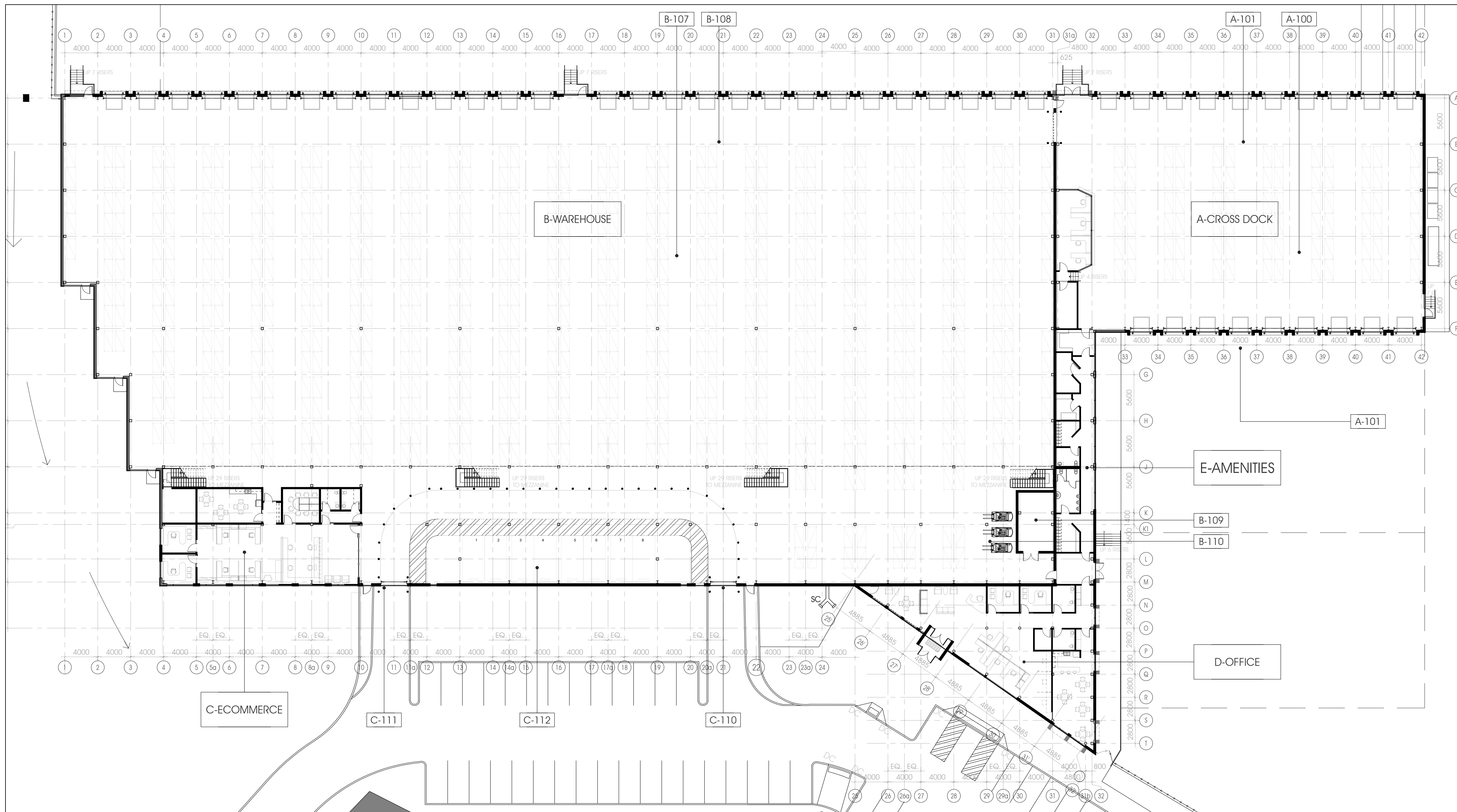
1 MAIN FLOOR PLAN A1.1 1:250
