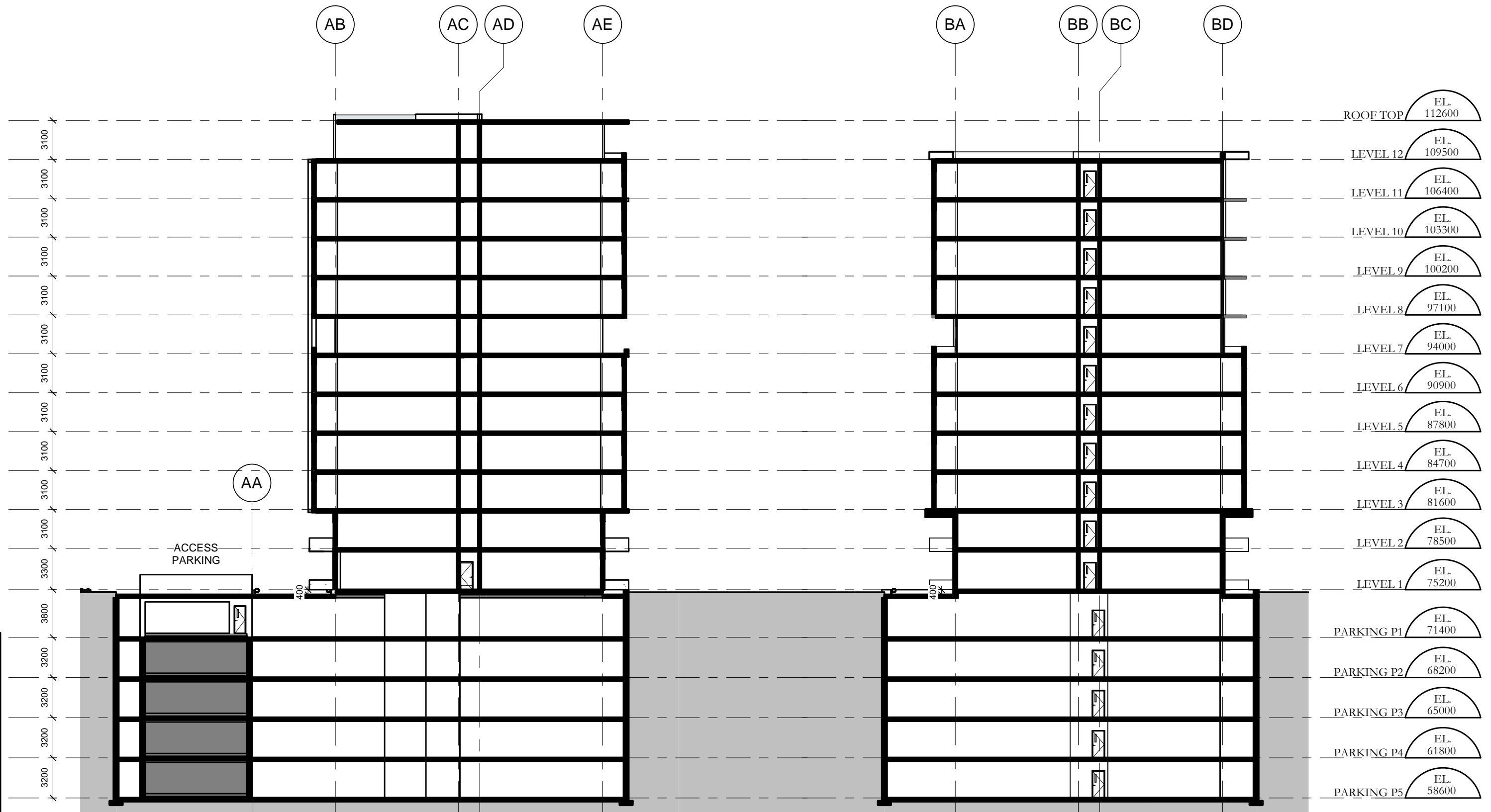
TOWER A - SECTION
