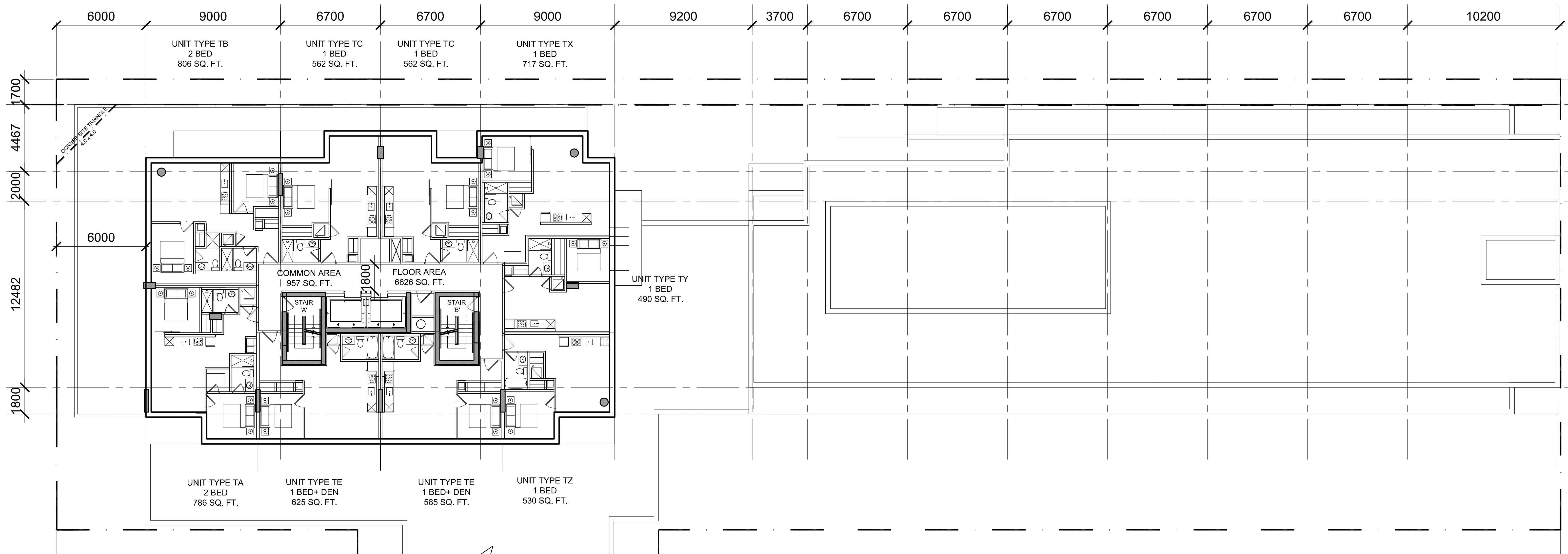
8TH - 17TH FLOOR PLAN
