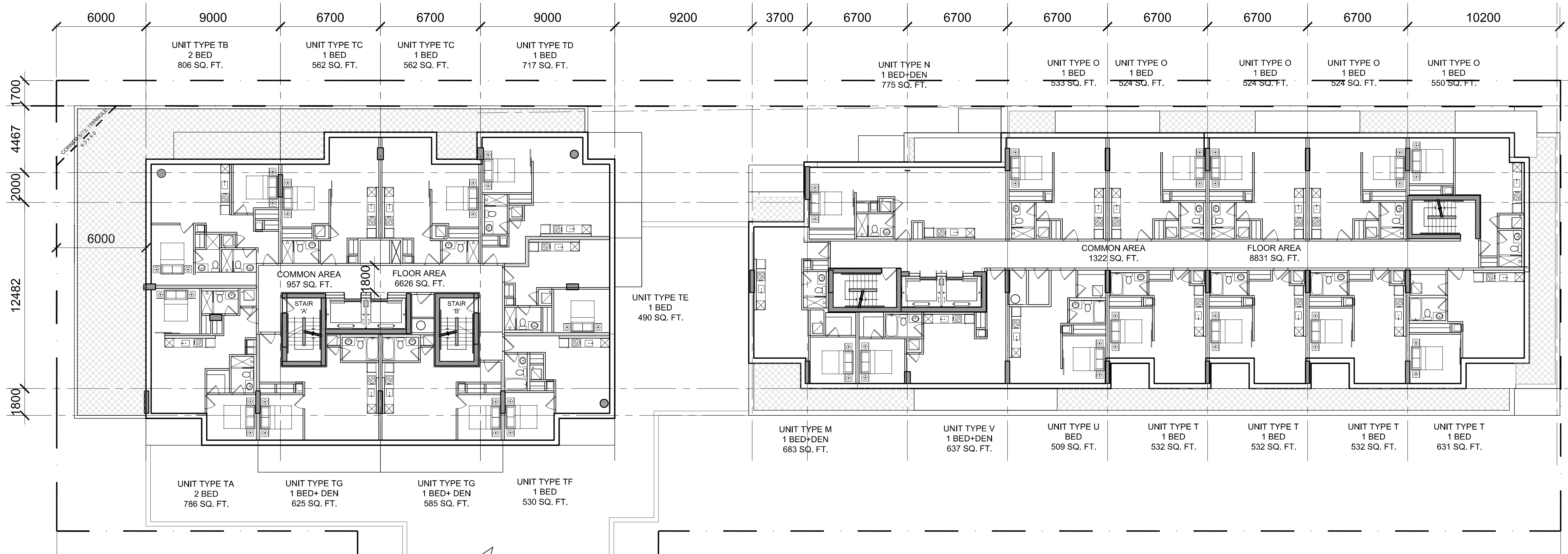
6TH - 7TH FLOOR PLAN
