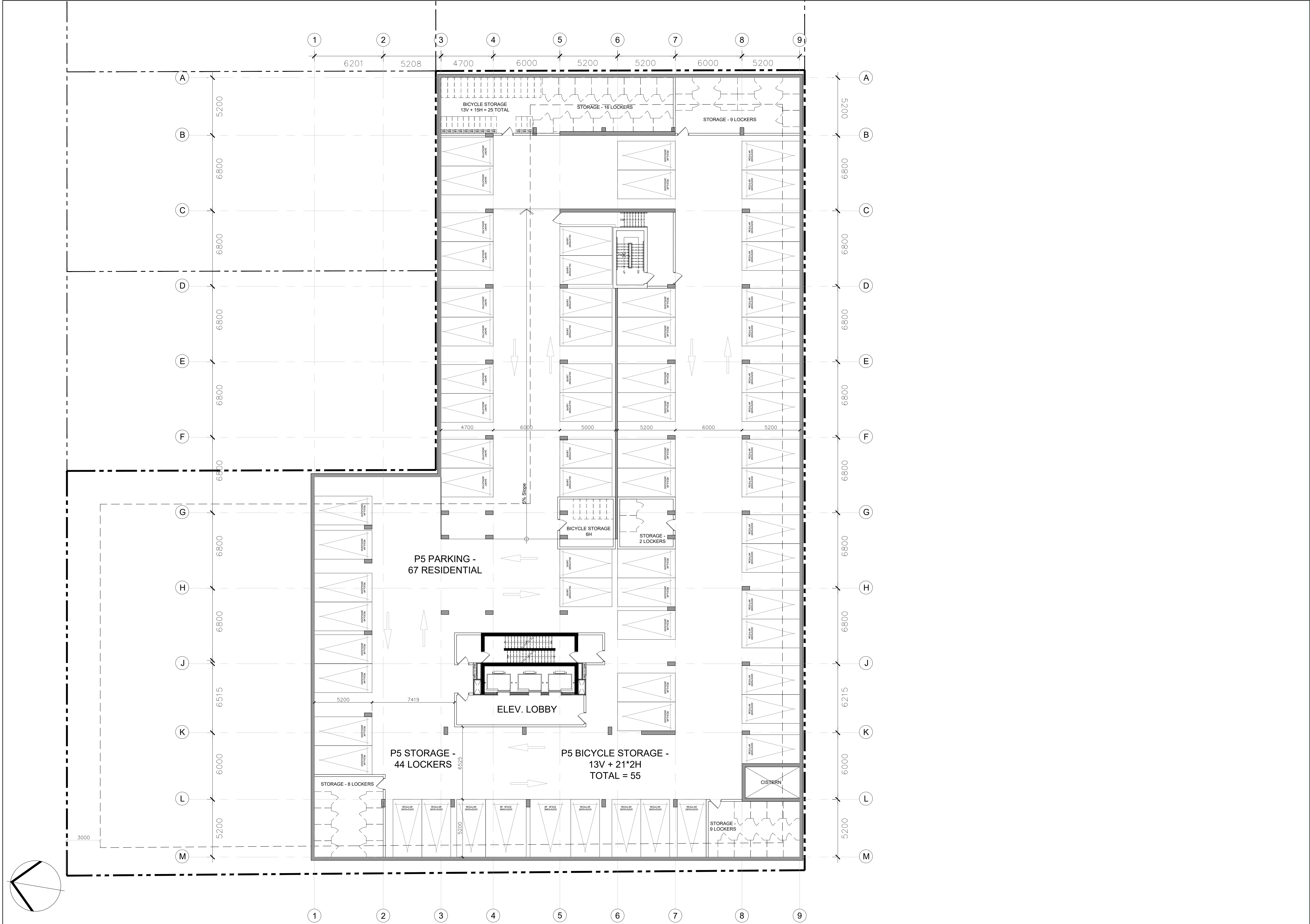
1 LEVEL P5 FLOOR PLAN A2.01 1:150
