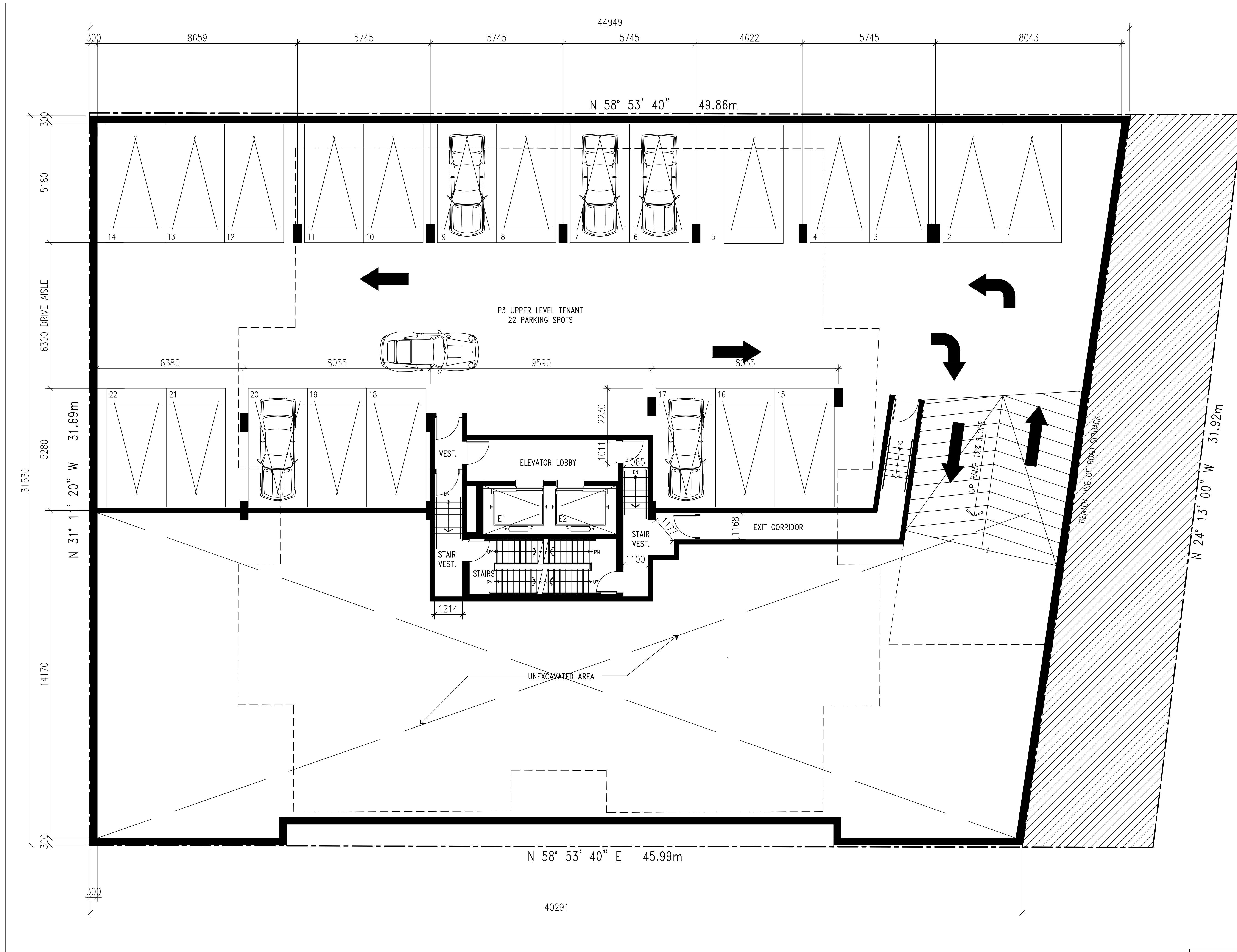
1 UPPER LEVEL 3-GARAGE FLOOR PLAN SCALE: 1:75
