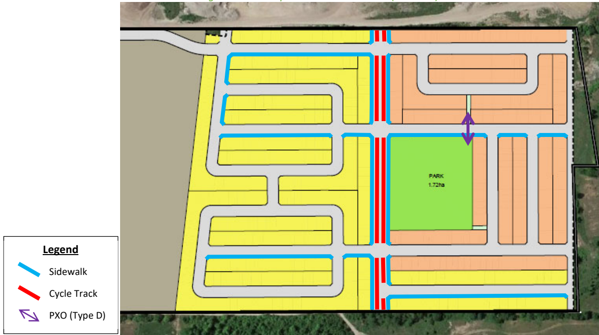
TIA Figure 11: Concept Pedestrian Network (REVISED)
