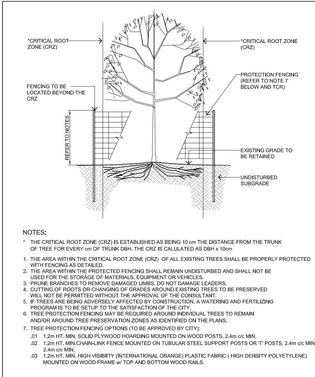
1:1.02 TREE PROTECTION BARRIER NTS
