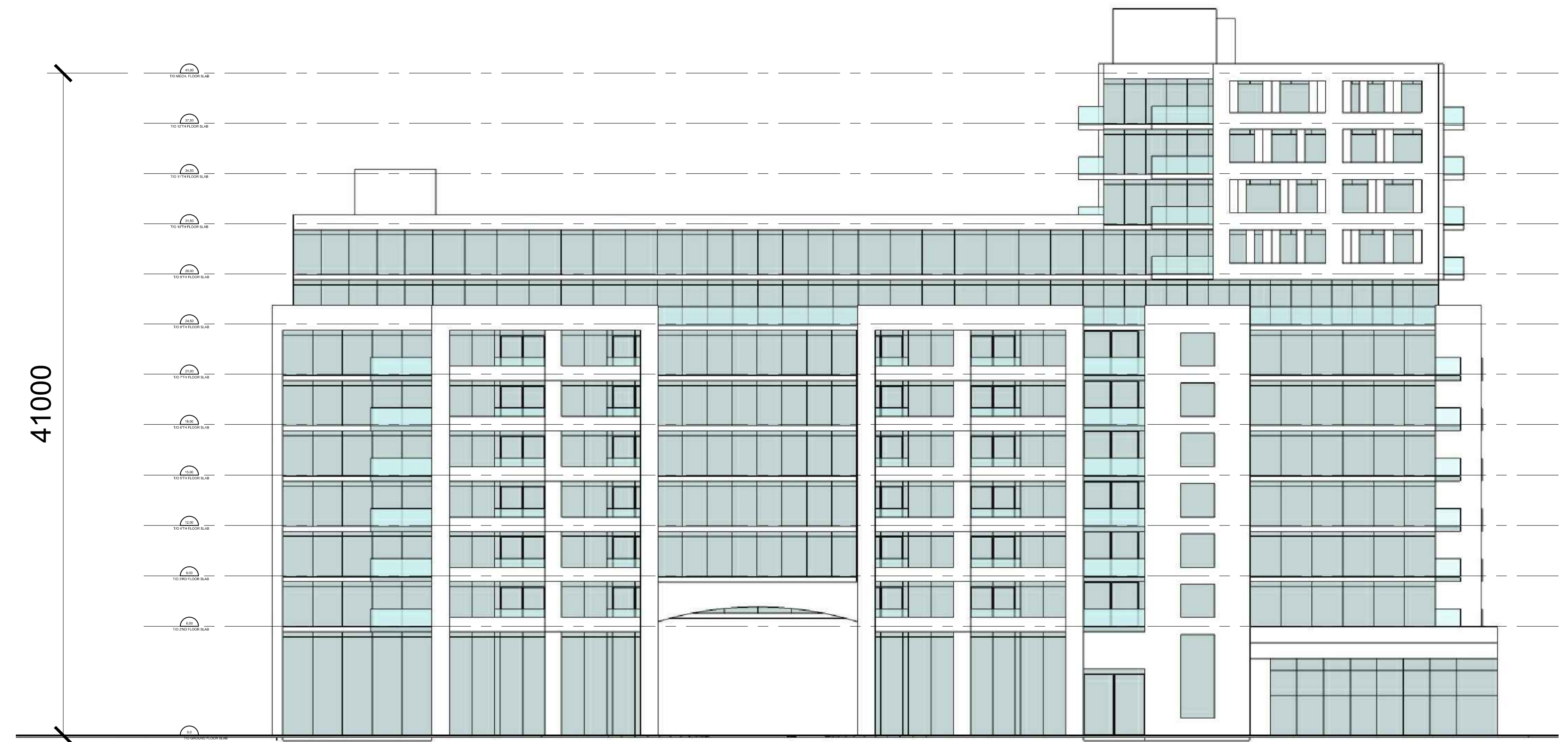
EAST ELEVATION
