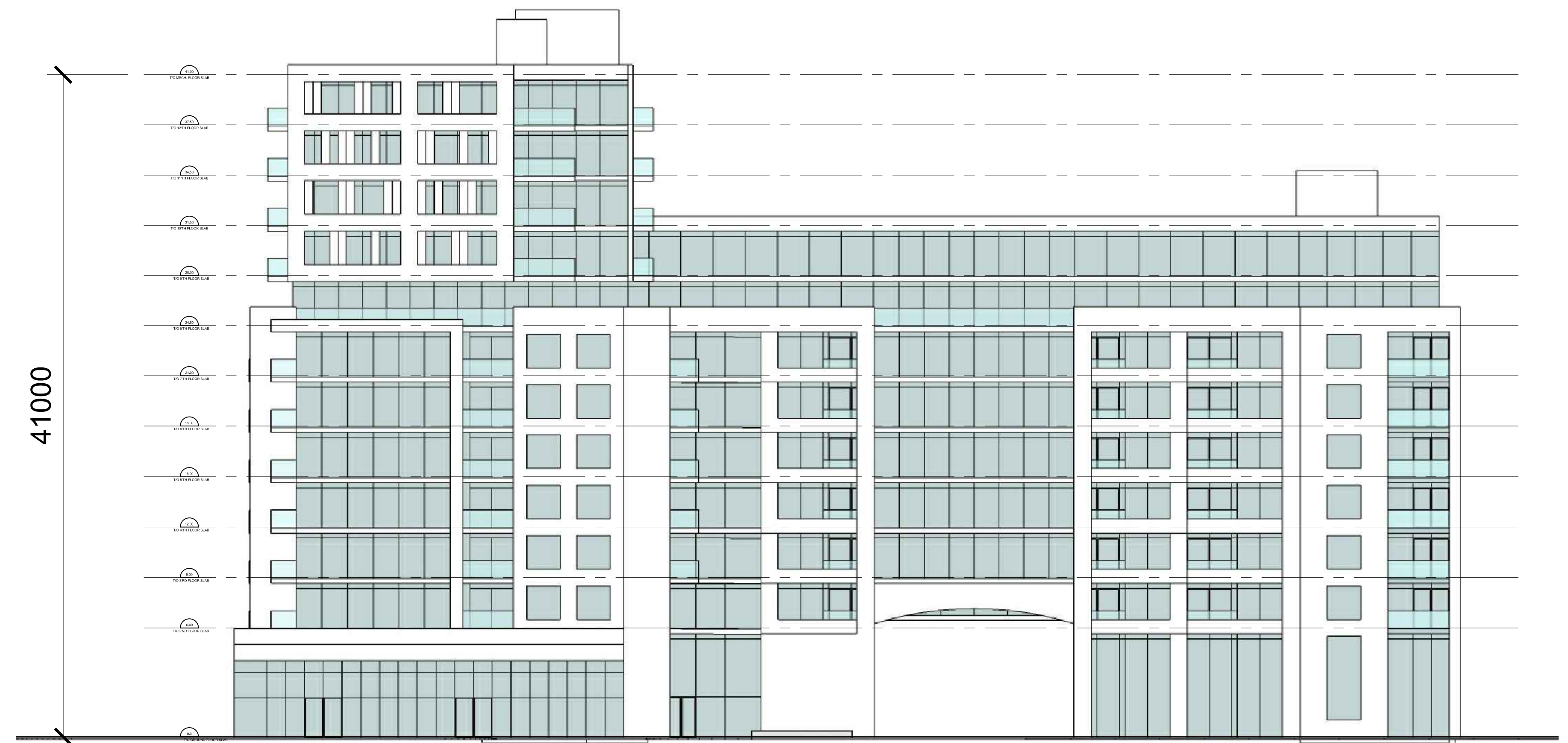
WEST ELEVATION
