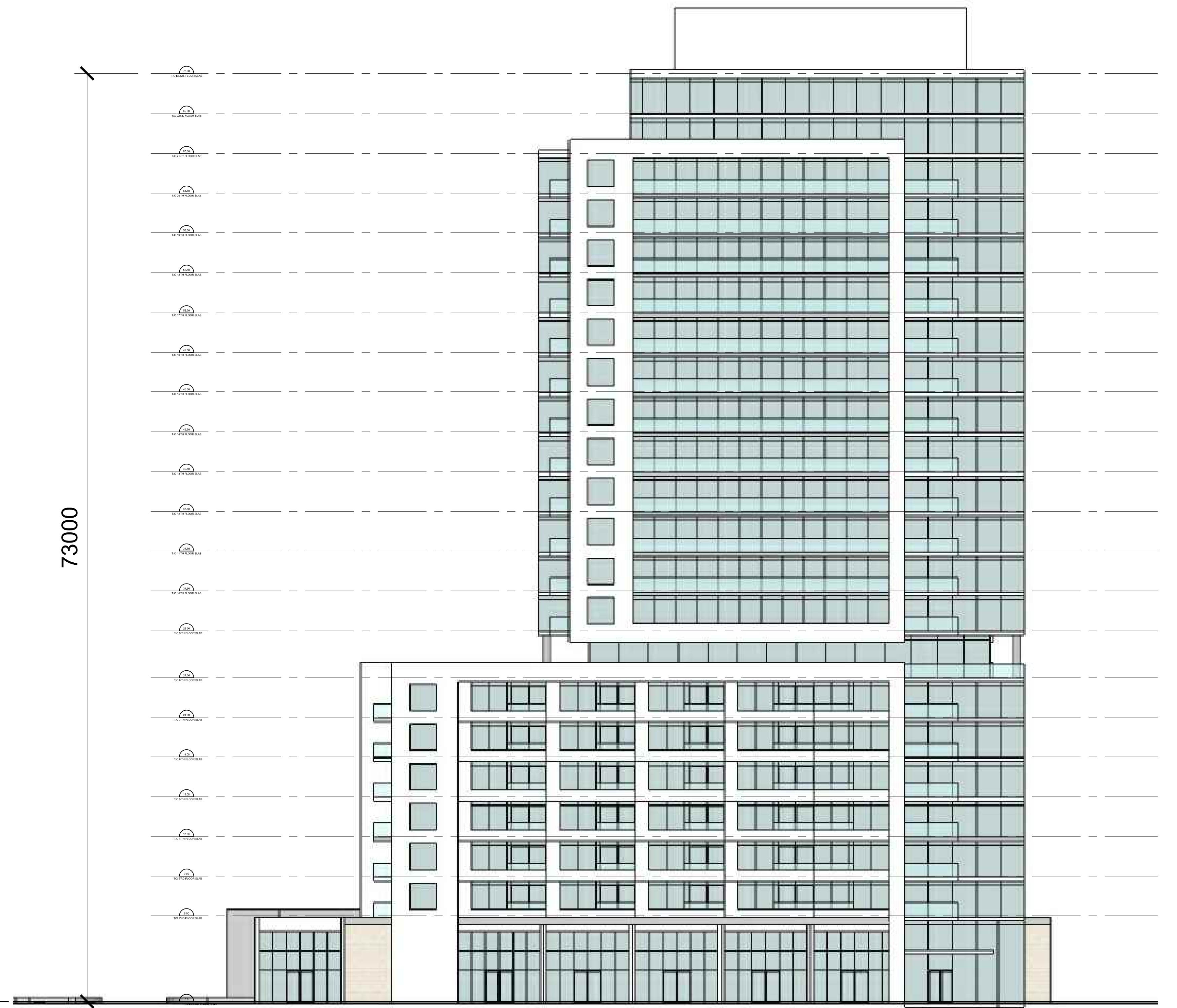
WEST ELEVATION
