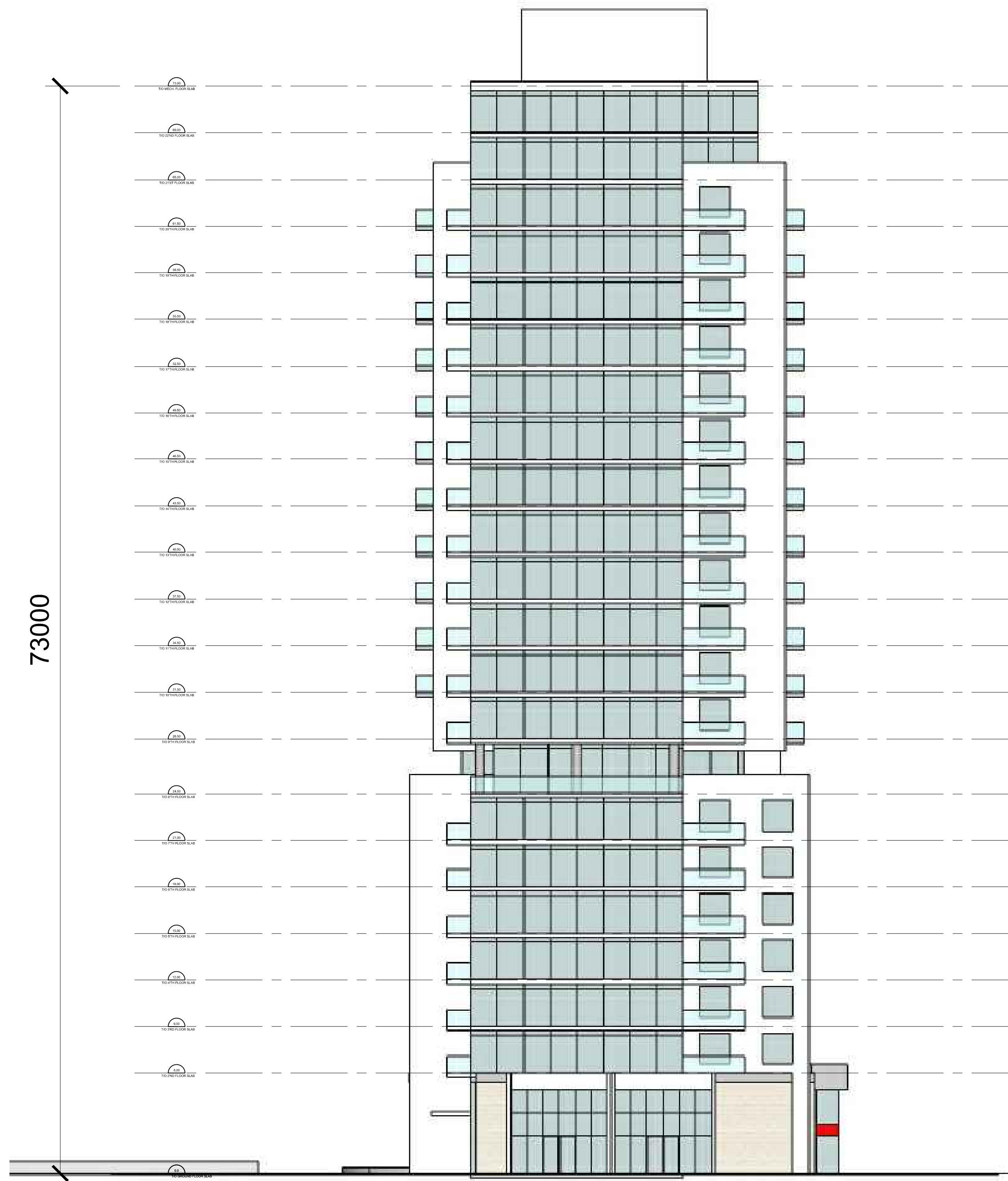
SOUTH ELEVATION
