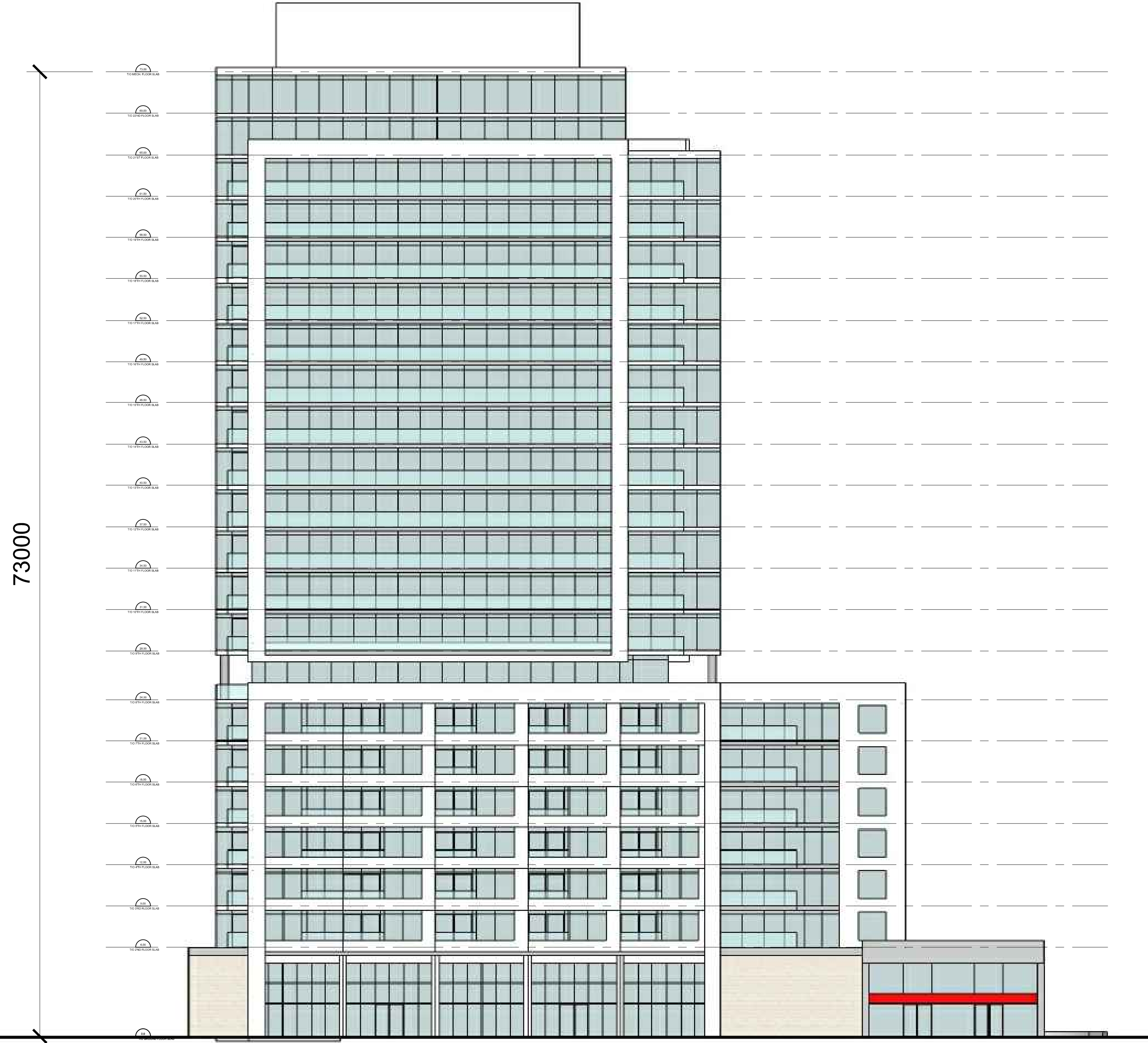
EAST ELEVATION
