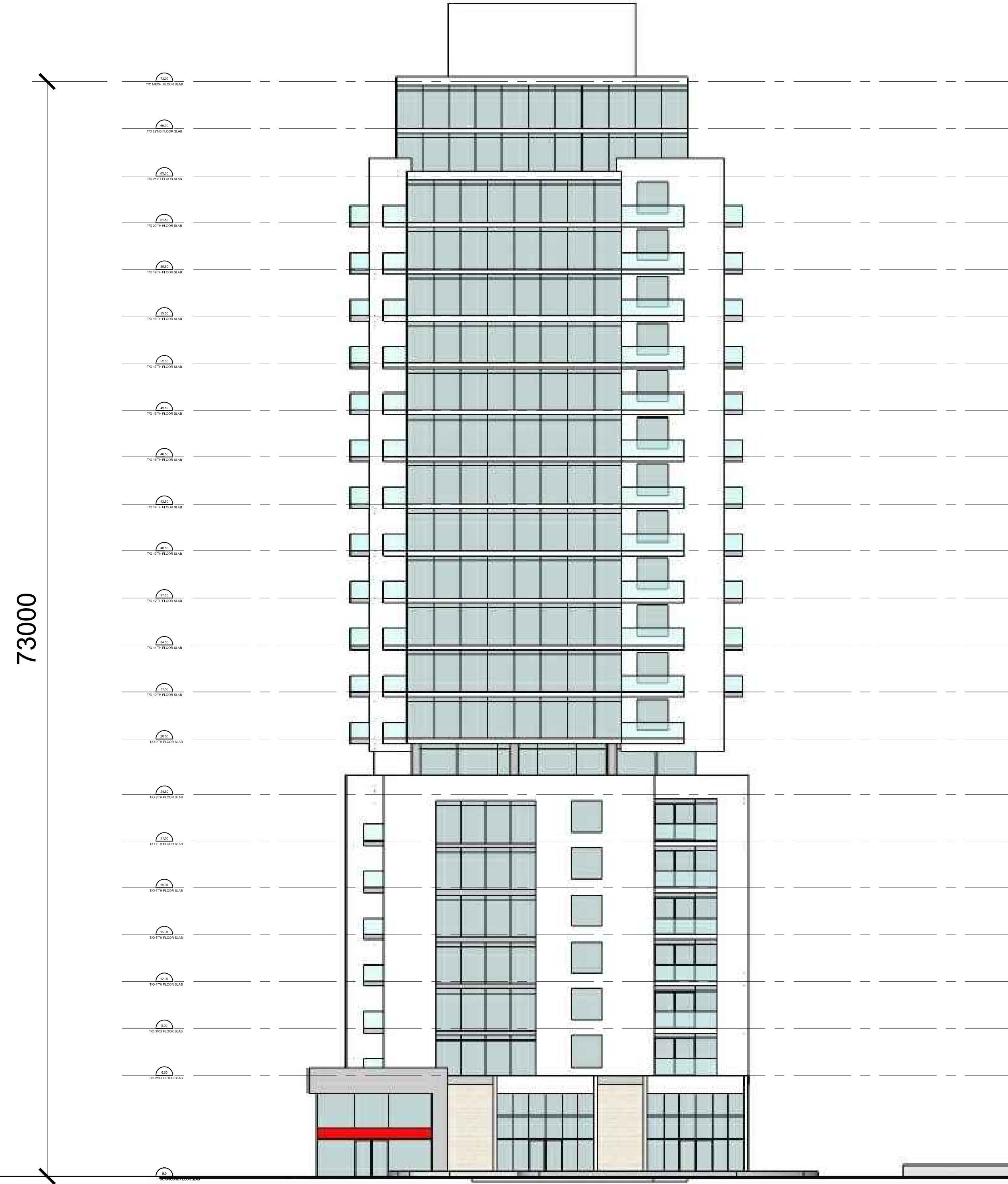
NORTH ELEVATION
