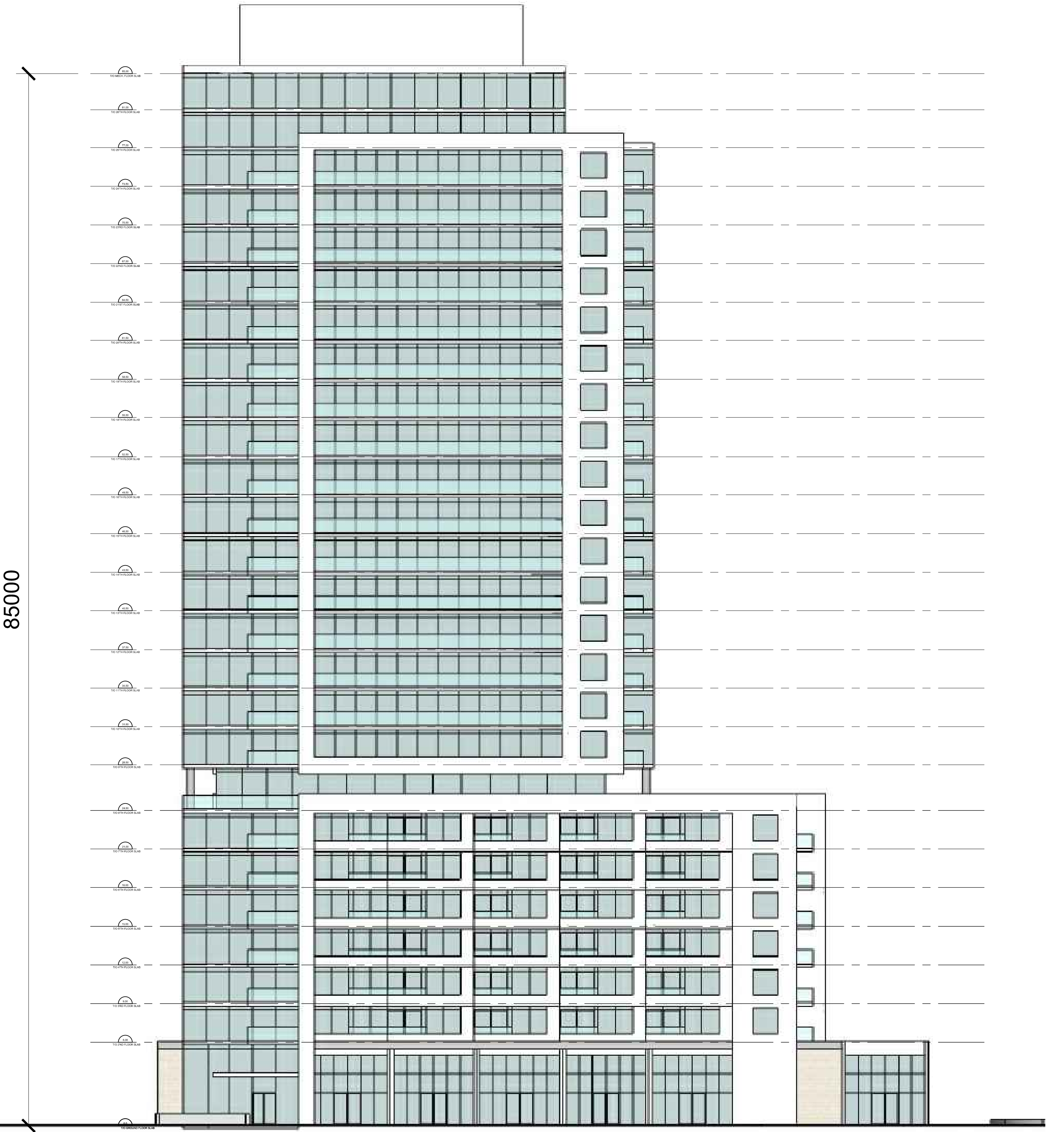
WEST ELEVATION
