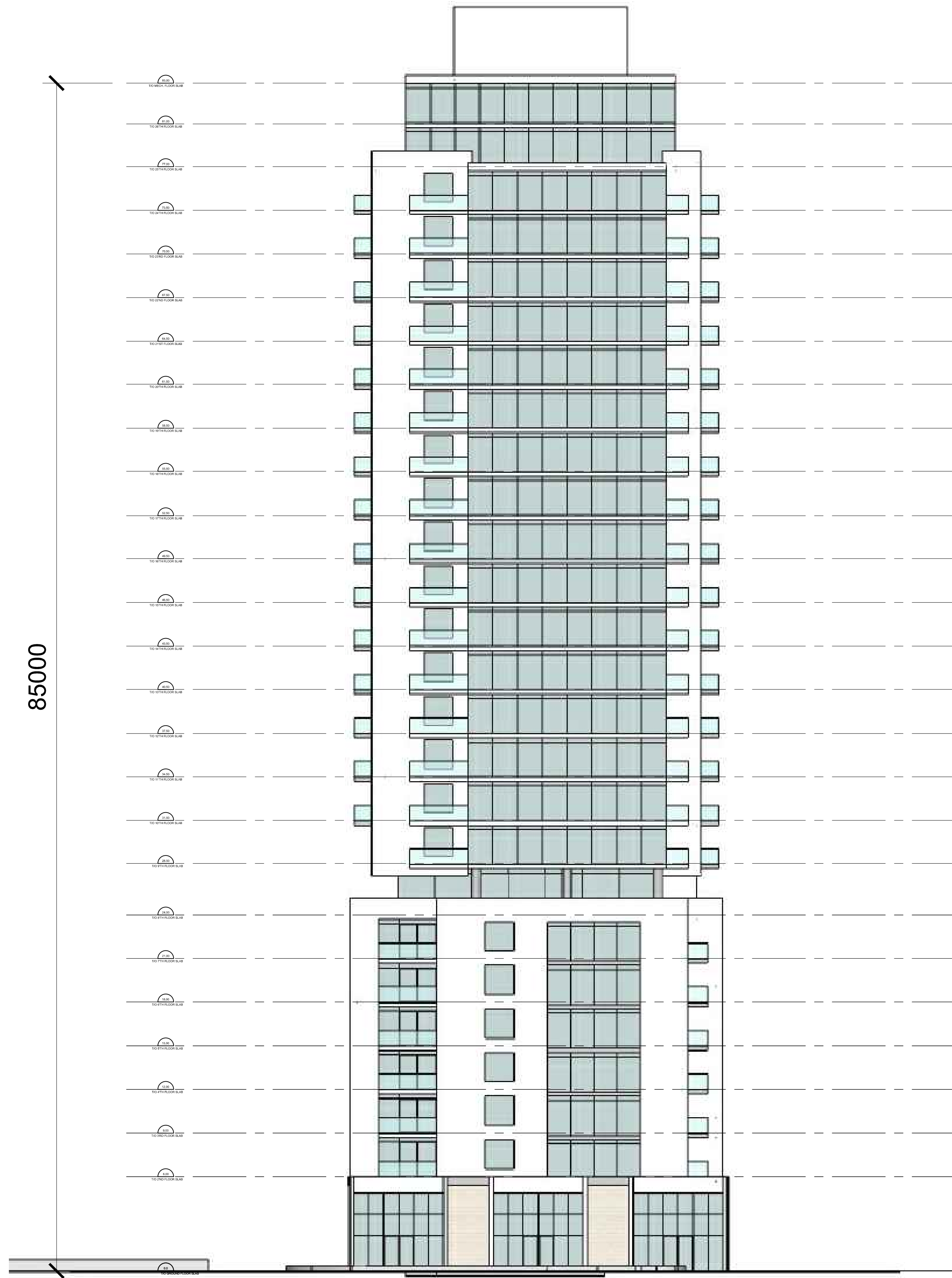
SOUTH ELEVATION
