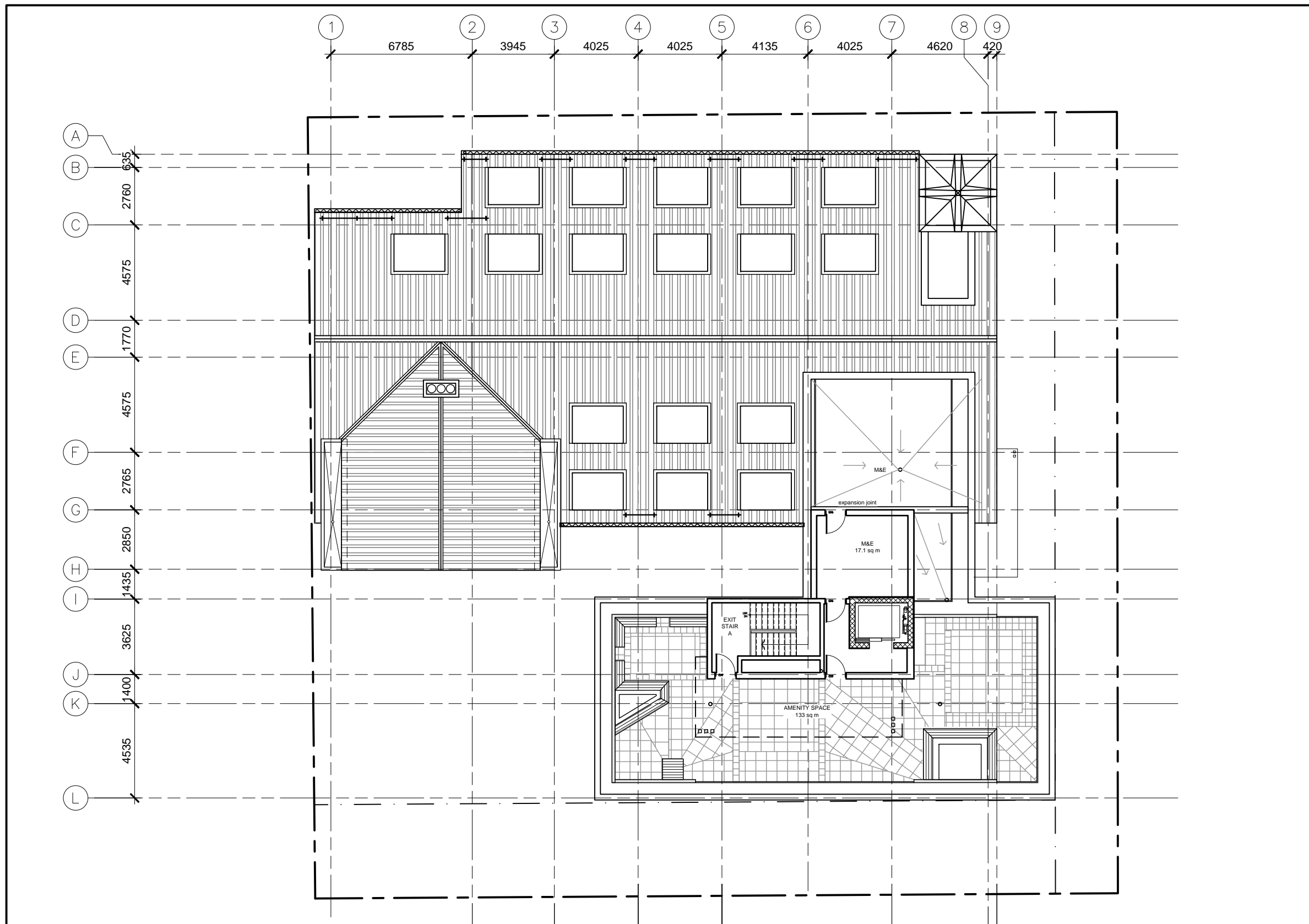
1 ROOF PLAN A5 1:200
