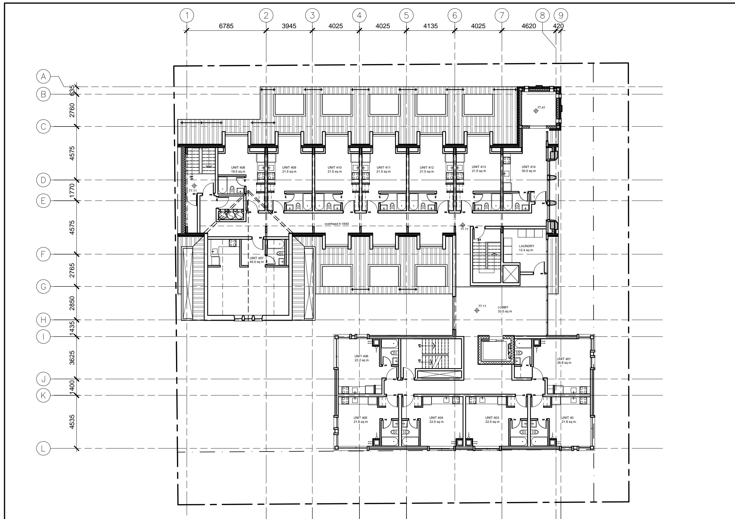
1 FOURTH FLOOR PLAN A4 1:200
