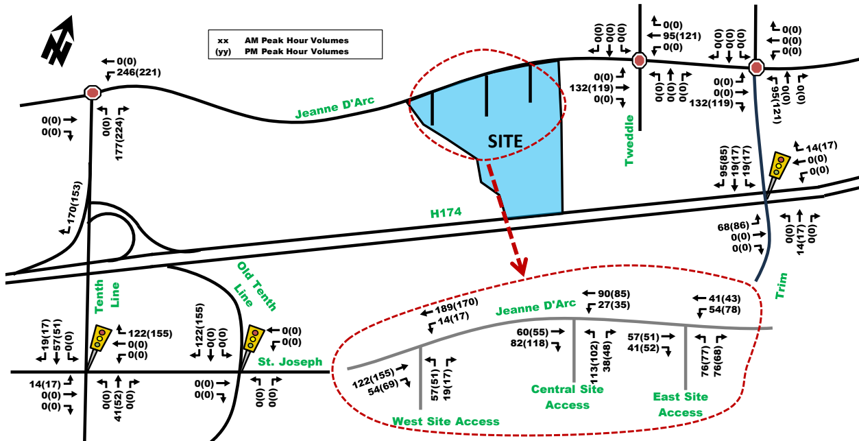
Figure 21: 'New' Site-Generated Traffic – Scenario 2 with Direct Connection to LRT
