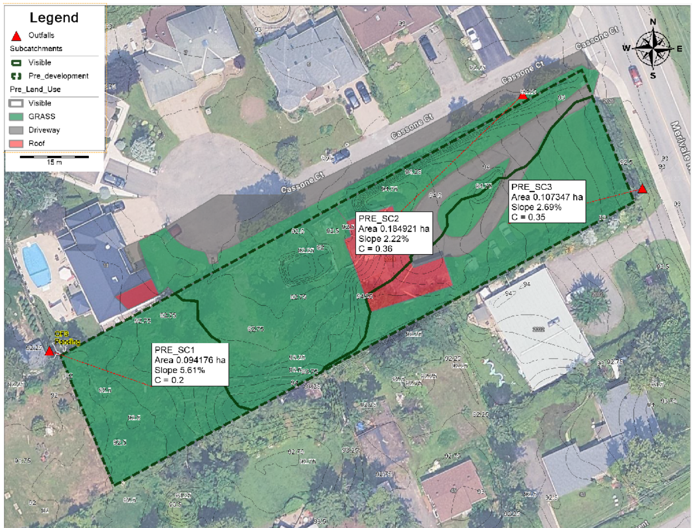
Figure 6-1 – Pre-development Sub-catchments
