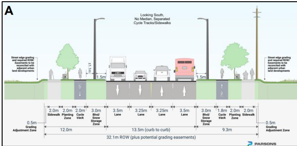
Figure 8: July 2025 TMP – Schedule D4 Urban Road Network
