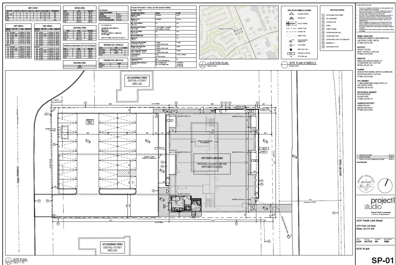
Figure 10. Site Plan
