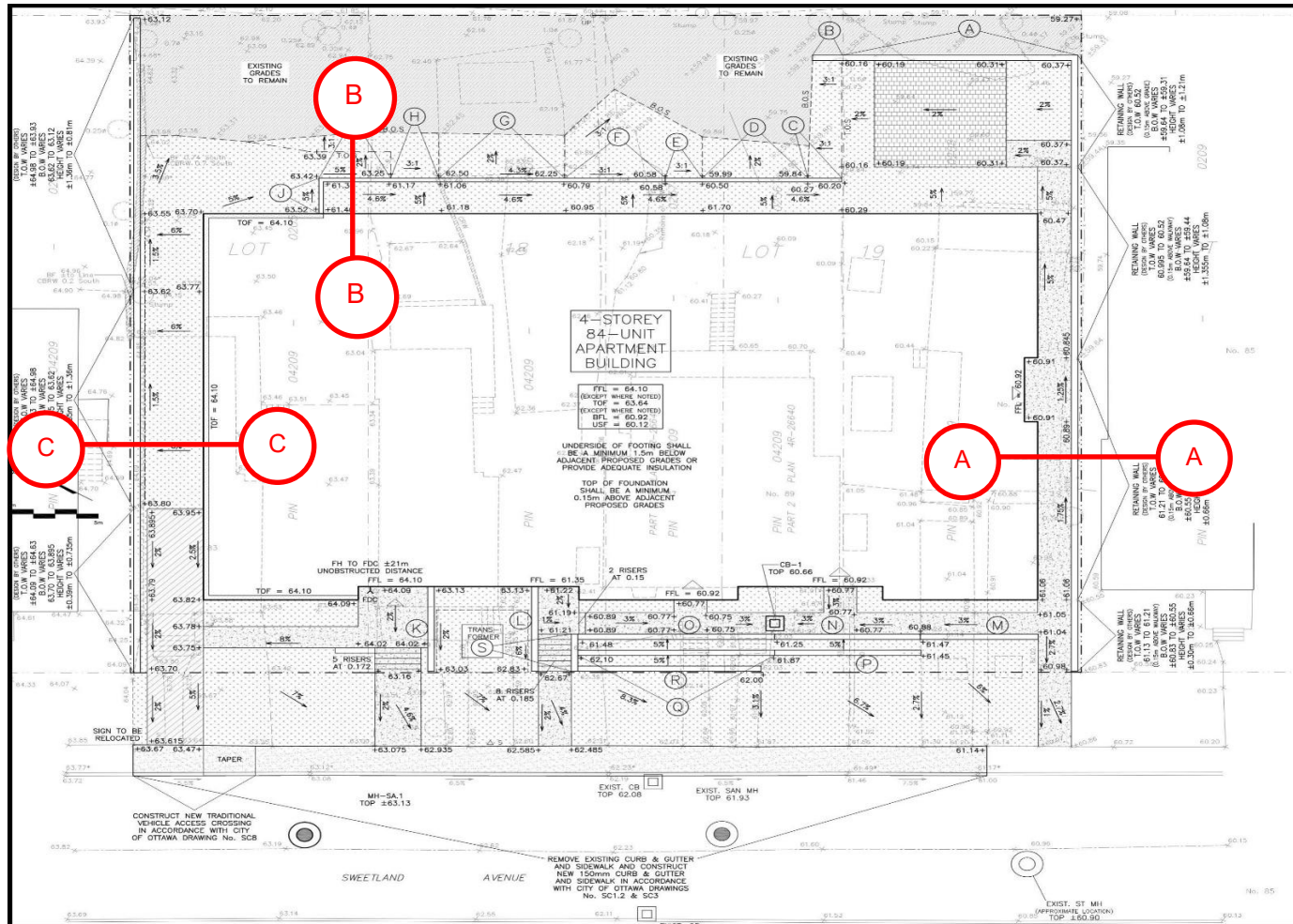
DRAWING PG7100-1
