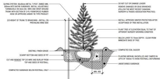
2 CONIFEROUS TREE PLANTING DETAIL 12 n.t.s.
