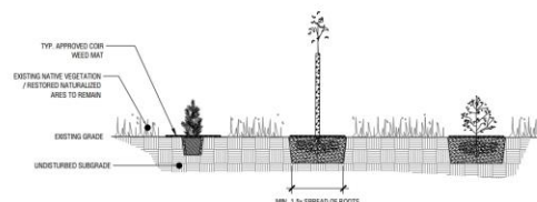
2 CONIFEROUS TREE PLANTING DETAIL 12 n.t.s.
