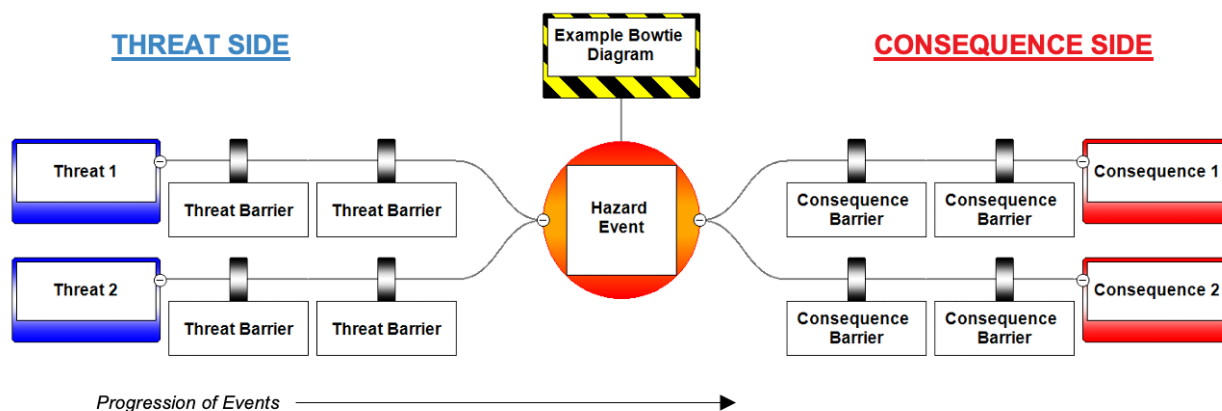
Figure 11 - Example Bowtie Diagram
