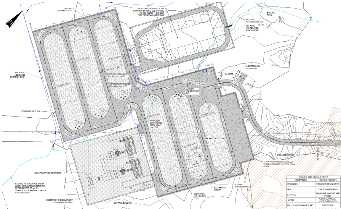
Figure 10 – Site Layout and Access
