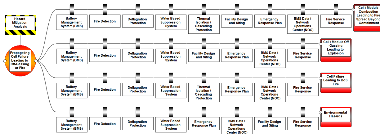
Figure 13 - Primary Consequence Barriers Diagram
