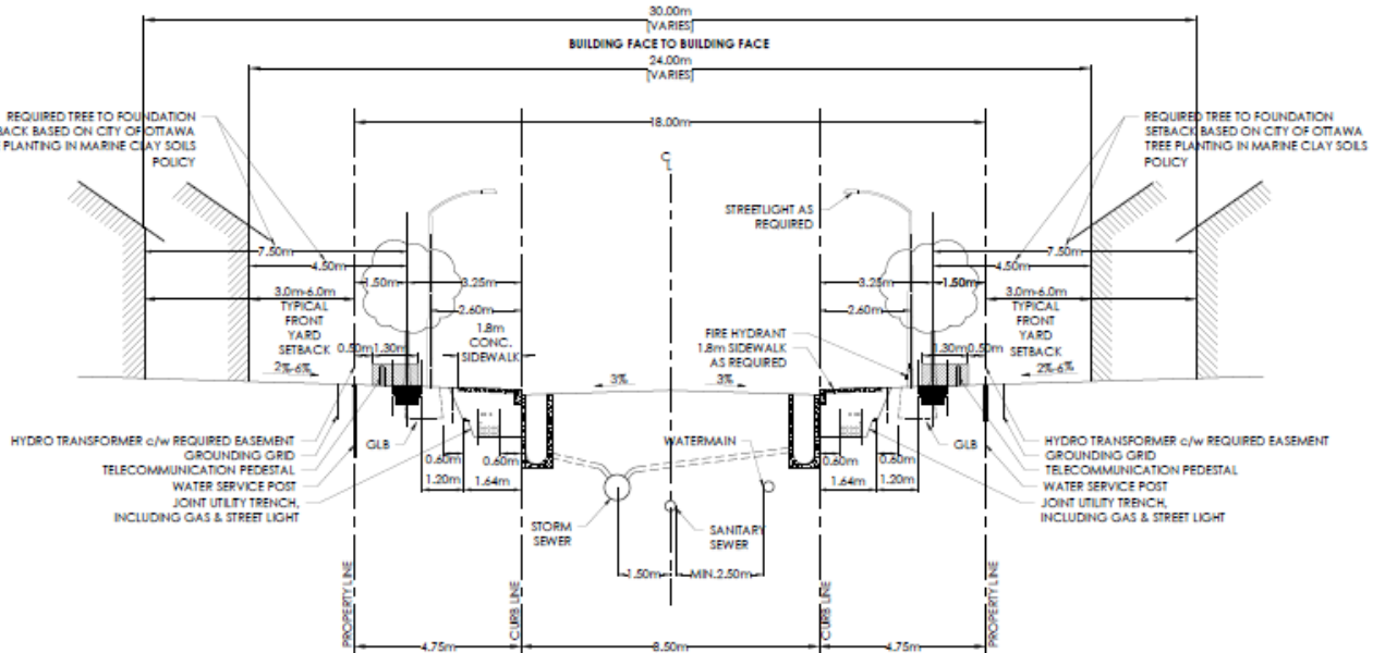
Figure 19. Typical 18m cross section
