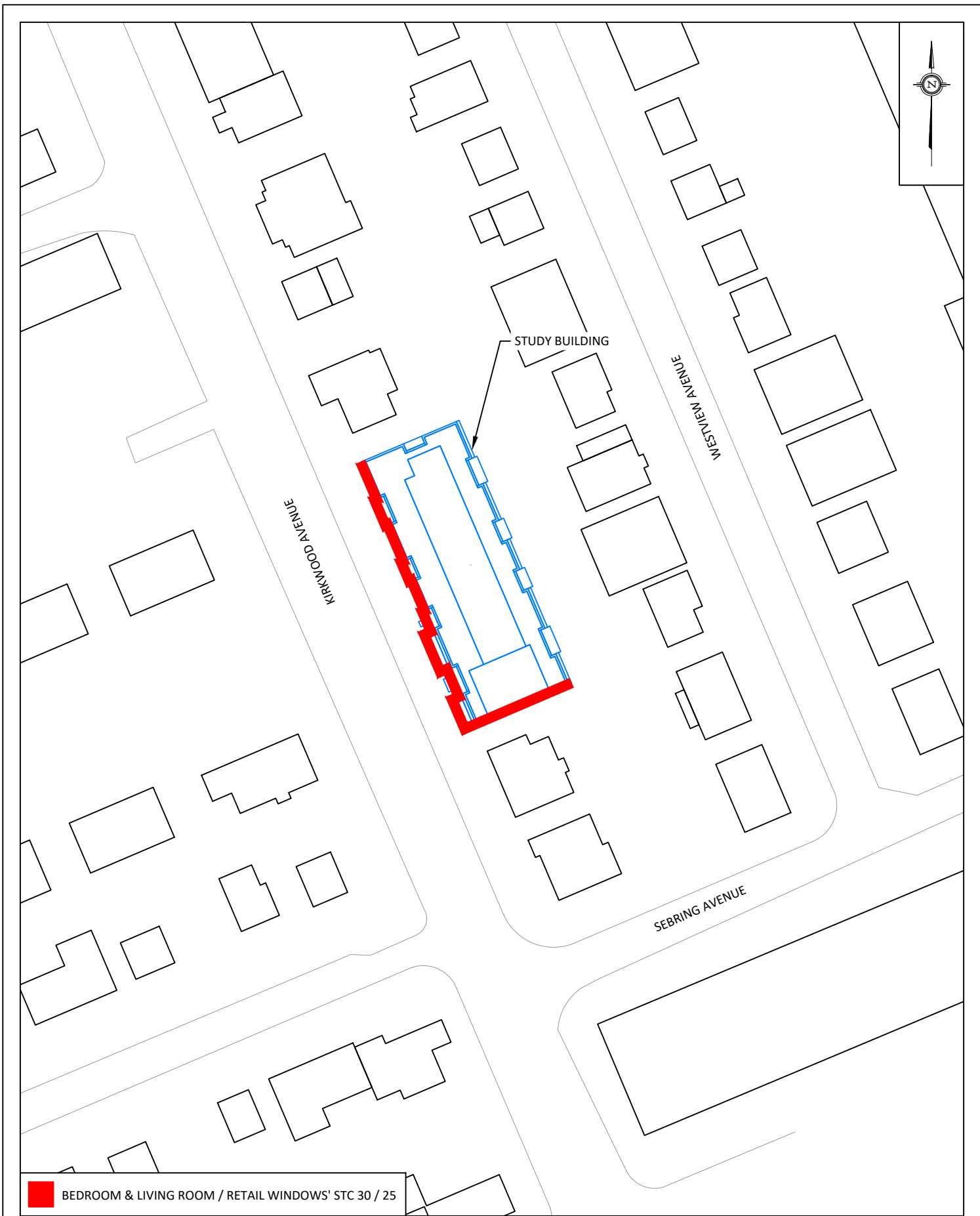
FIGURE 3: STC REQUIREMENTS
