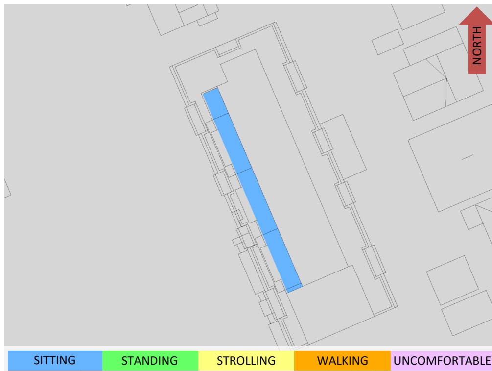
FIGURE 7B: SUMMER – WIND COMFORT, PH LEVEL AMENITY TERRACE
