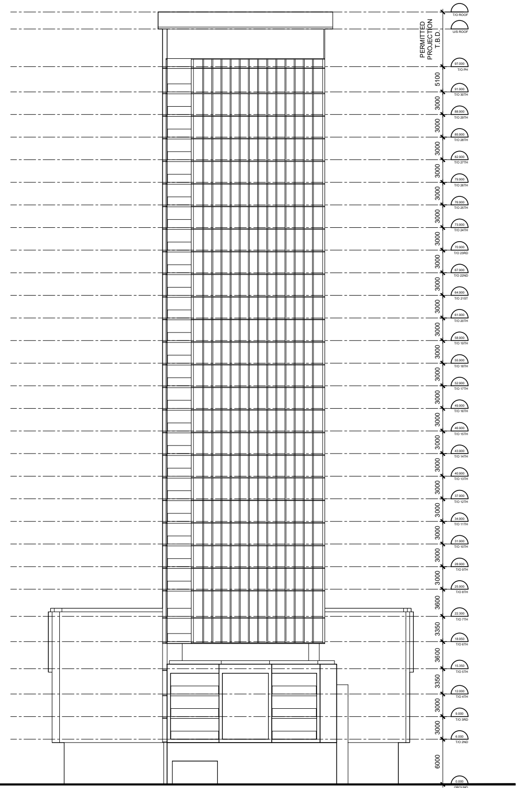
PHASE 1 - NORTH ELEVATION
