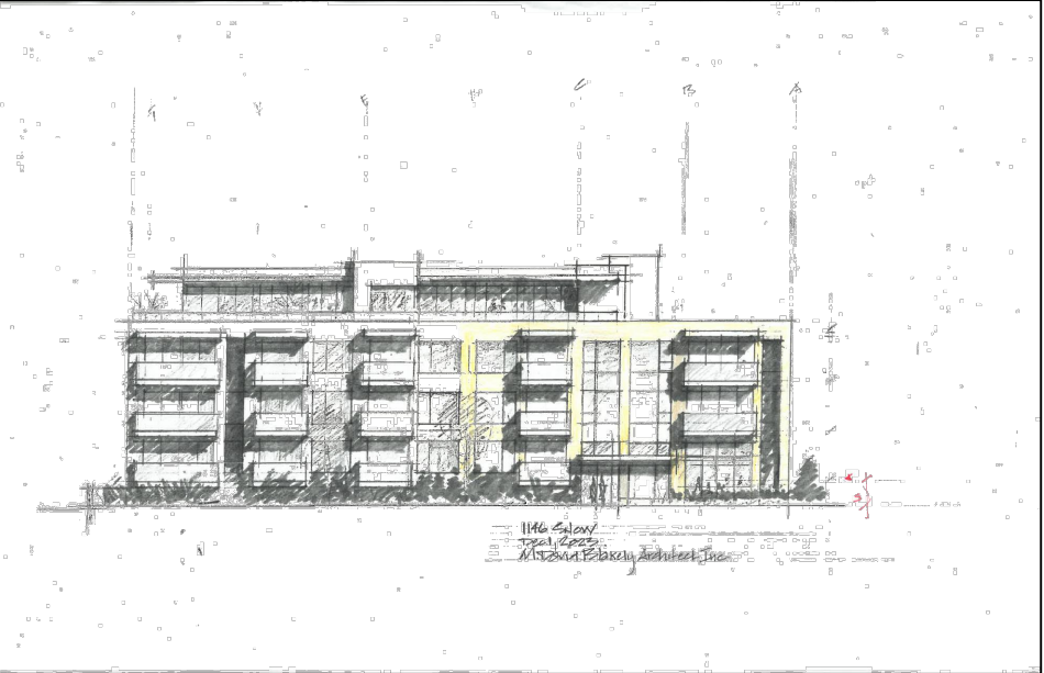
(4) 4- STOREY APARTMENT SKETCH ELEVATION NOVEMBER 22nd, 2023 - 36 UNIT DEVELOPMENT
