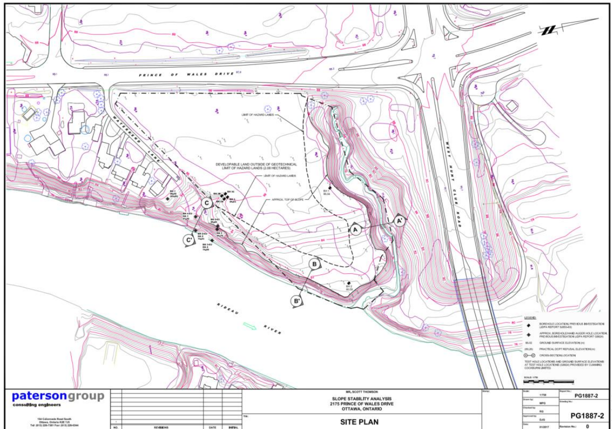
Figure 6 Slope Stability Analysis Setbacks (Paterson Group, 2017)
