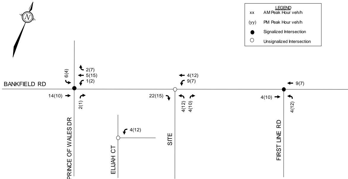
Figure 3: Site-Generated Volumes
