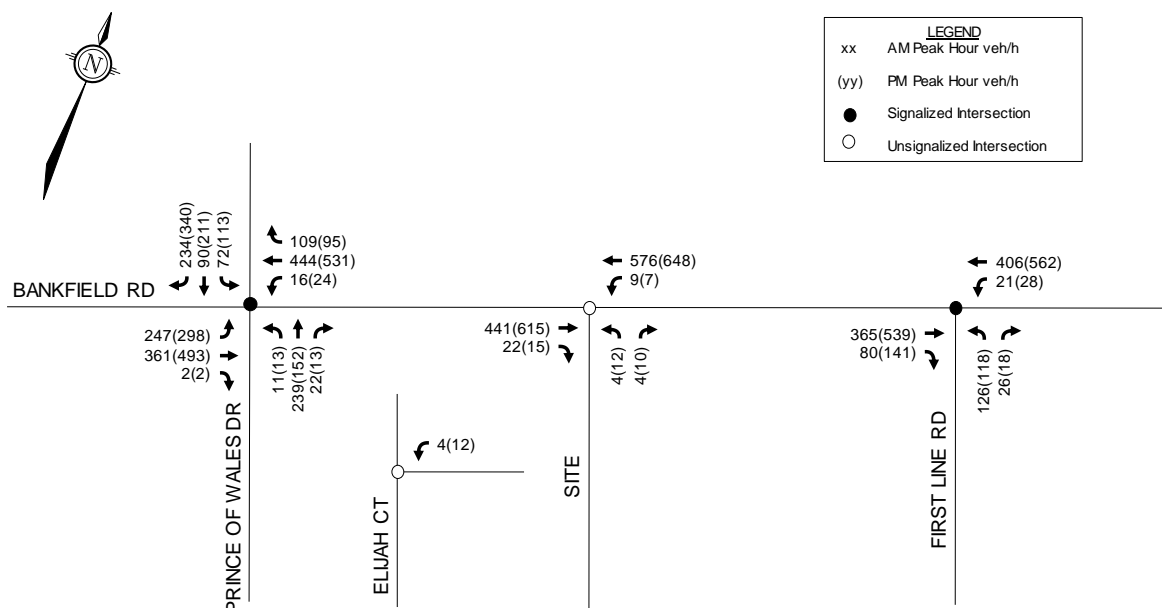
Figure 7: 2030 Total Traffic
