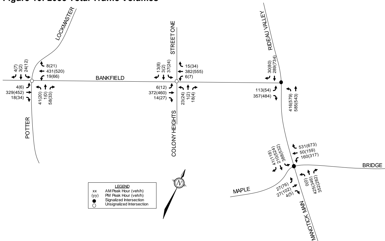
Figure 10: 2033 Total Traffic Volumes
