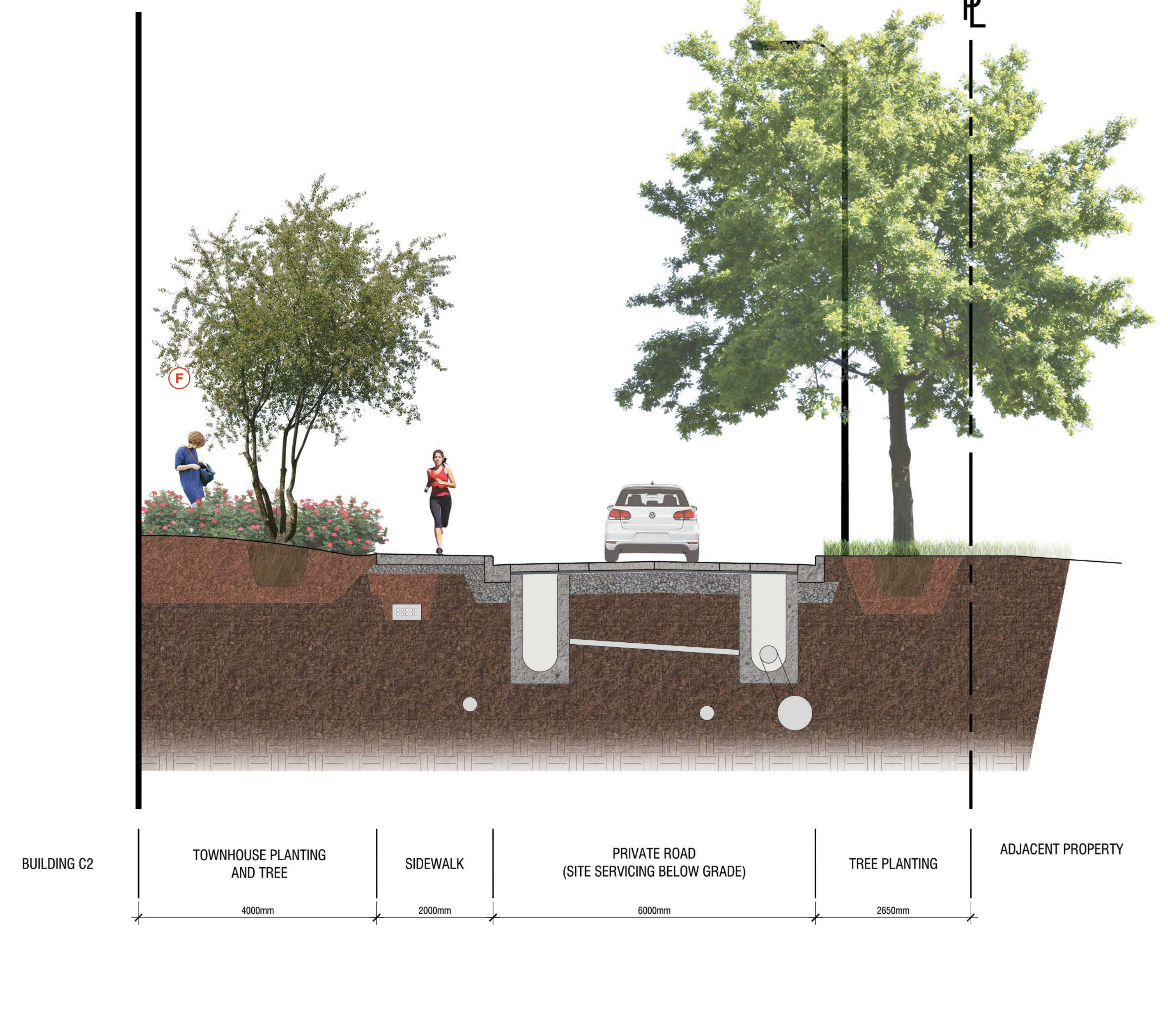
2 SECTION B-B AT PRIVATE ROAD L2 1:50
