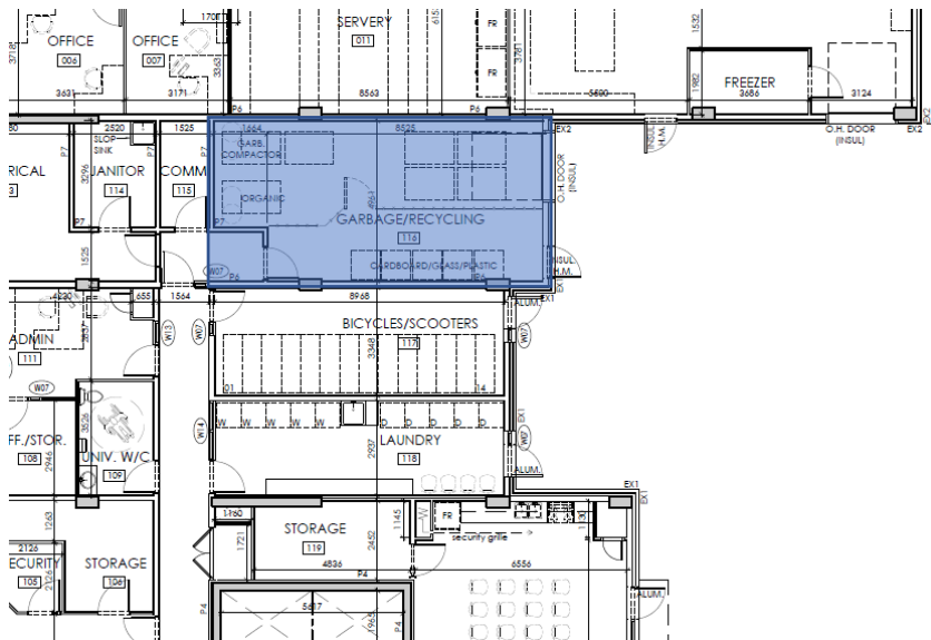
Figure 41. Excerpt from Ground Floor Plan Showing Interior Residential Waste Storage
