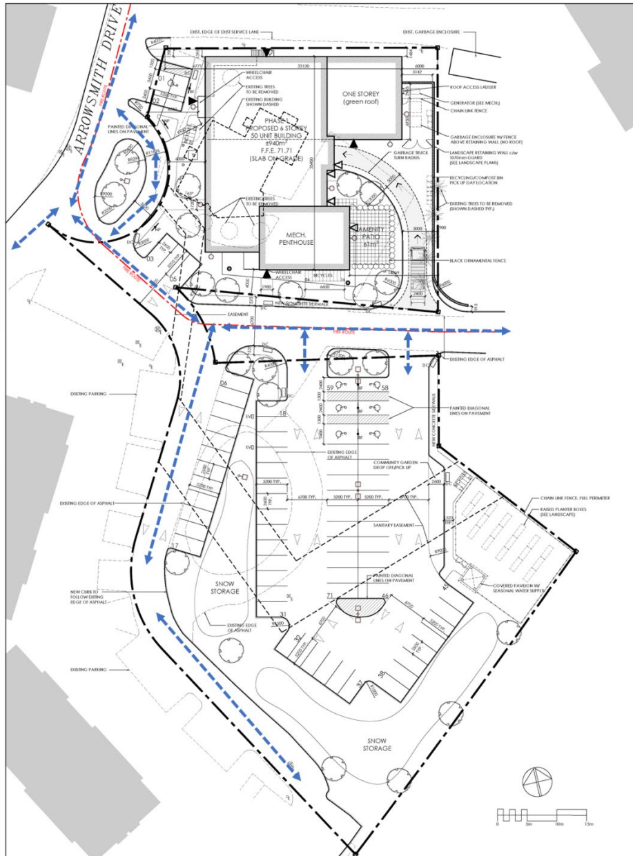
Figure 39. Excerpt from Site Plan Showing Automobile Circulation (Blue)
