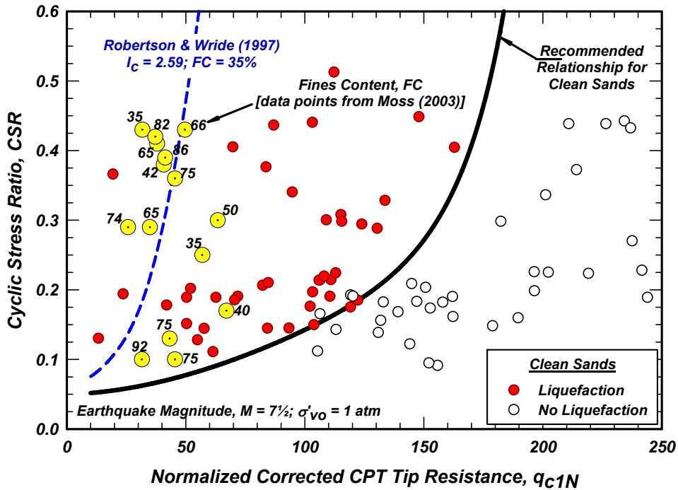
FIG. 2-5: Comparison of field case histories for silty sands, sandy silts, and silts and the curve proposed by Robertson & Wride (1997) for soils with l_c = 2.59 (apparent FC = 35\% ) [Idriss and Boulanger 2004].
