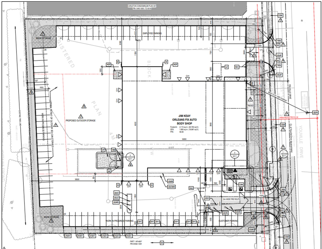
Figure 2.1 Proposed Development
