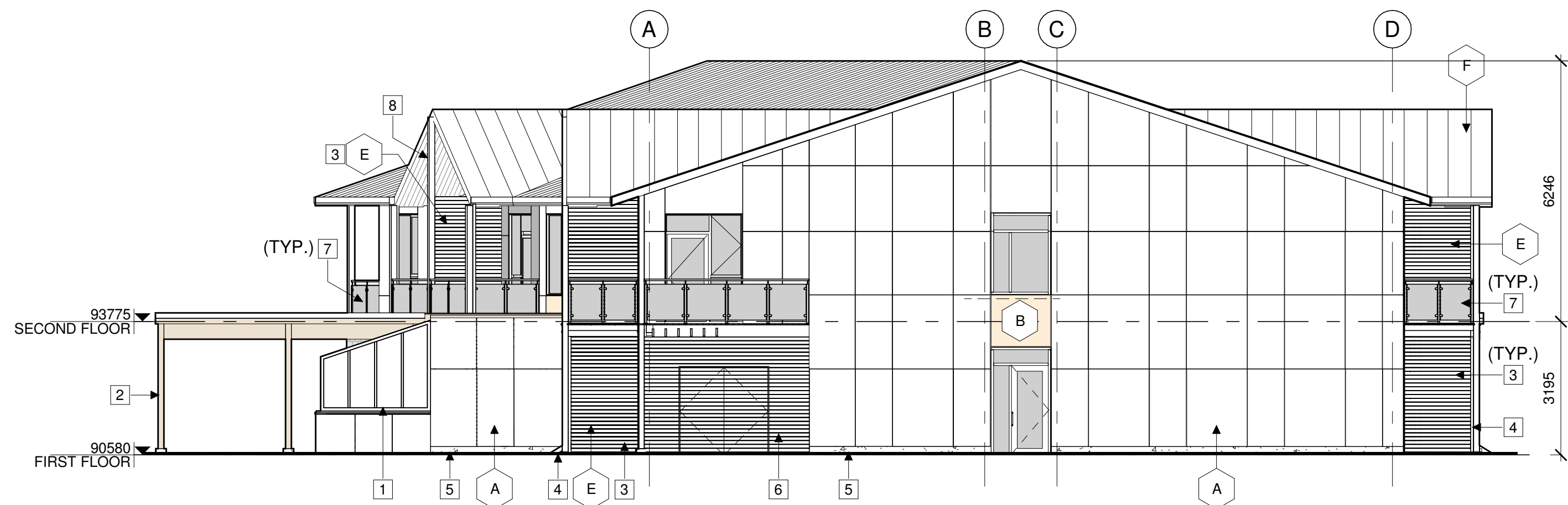
5 WEST ELEVATION
