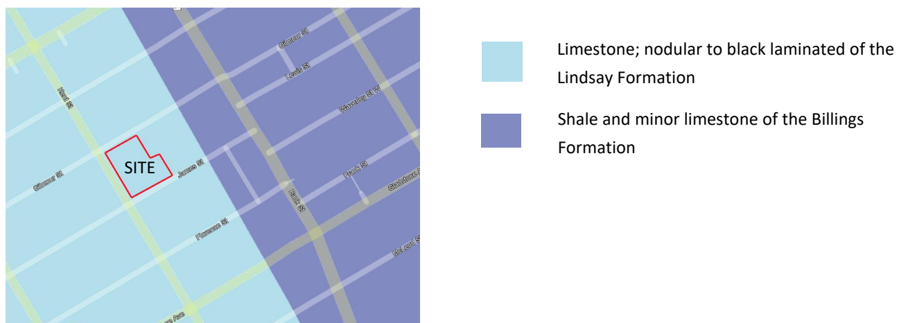
Image 2 – Bedrock Geology
