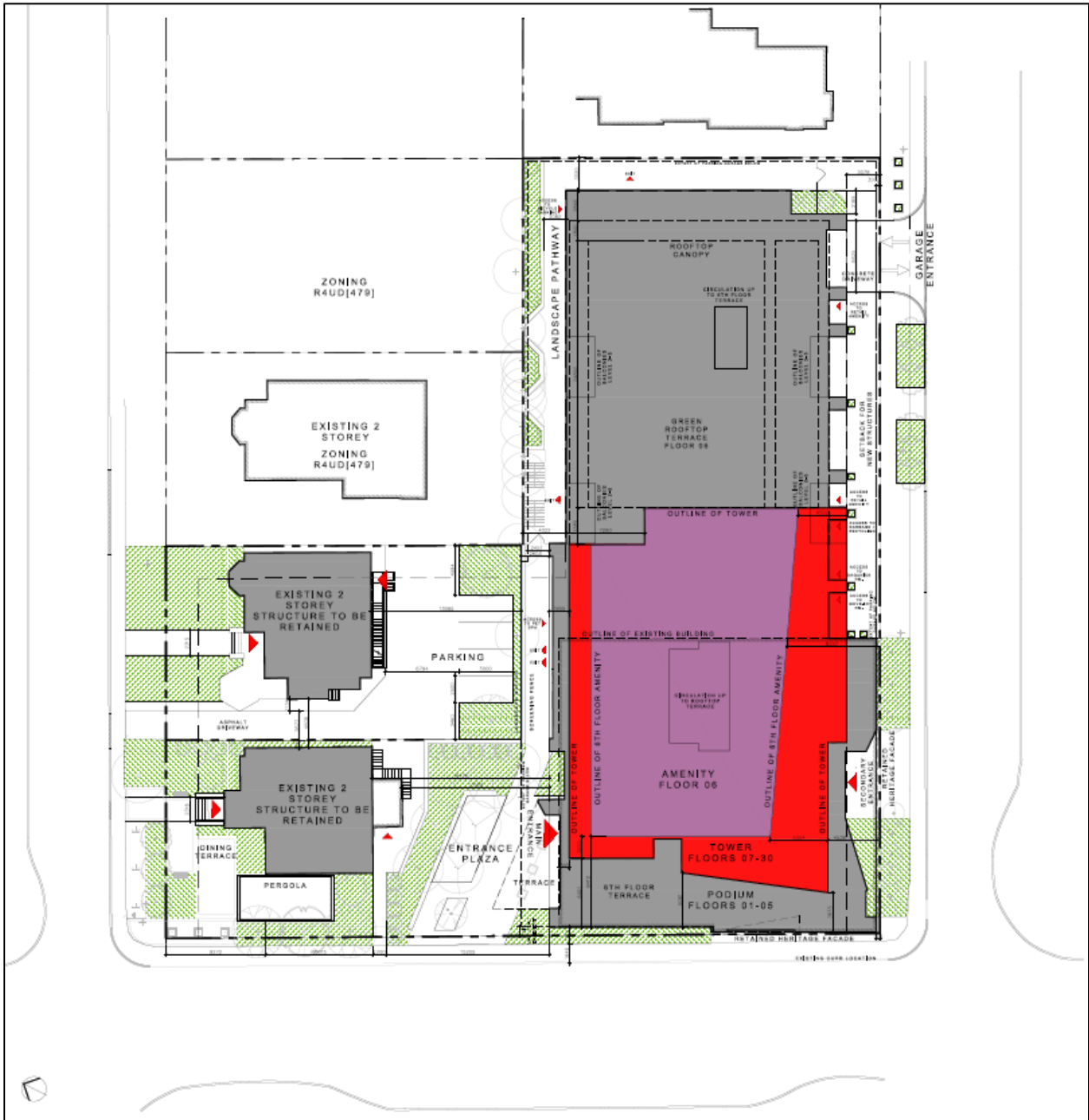
Figure 3: Proposed 359 Kent Site Concept (February 2023)
