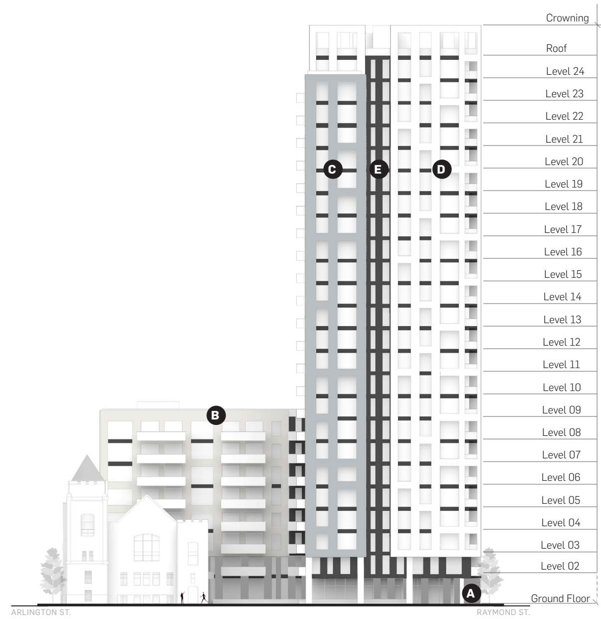
WEST / BELL STREET 1:500
