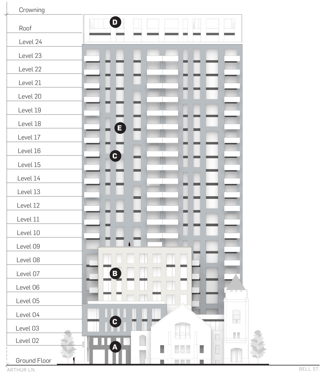
NORTH / ARLINGTON STREET 1:500
