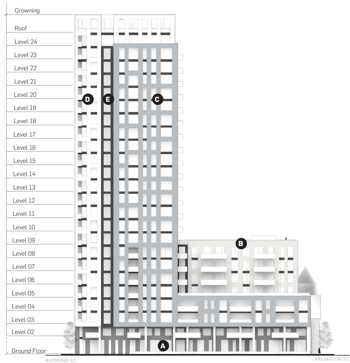
EAST / ARTHUR LANE 1:500
