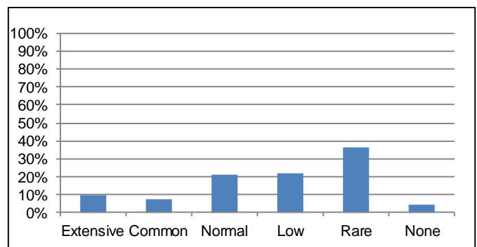
Figure 18 Instream vegetation abundance in Stillwater Creek
