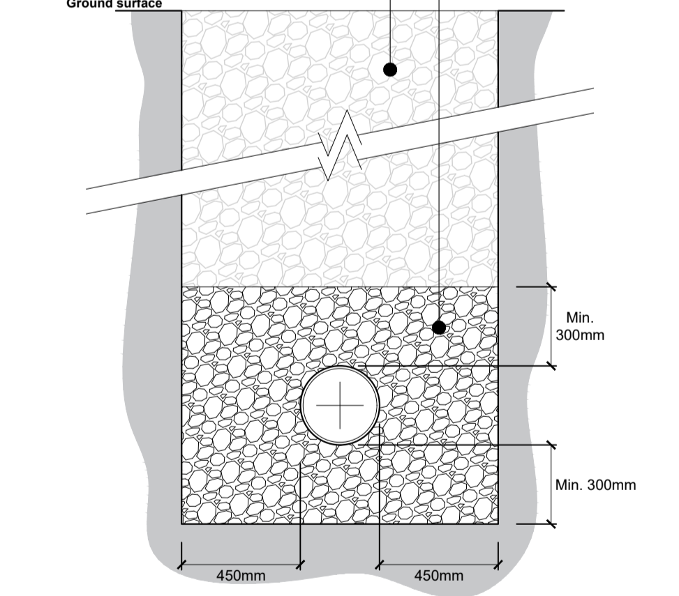
1 Standard Trench Detail Scale: As shown
