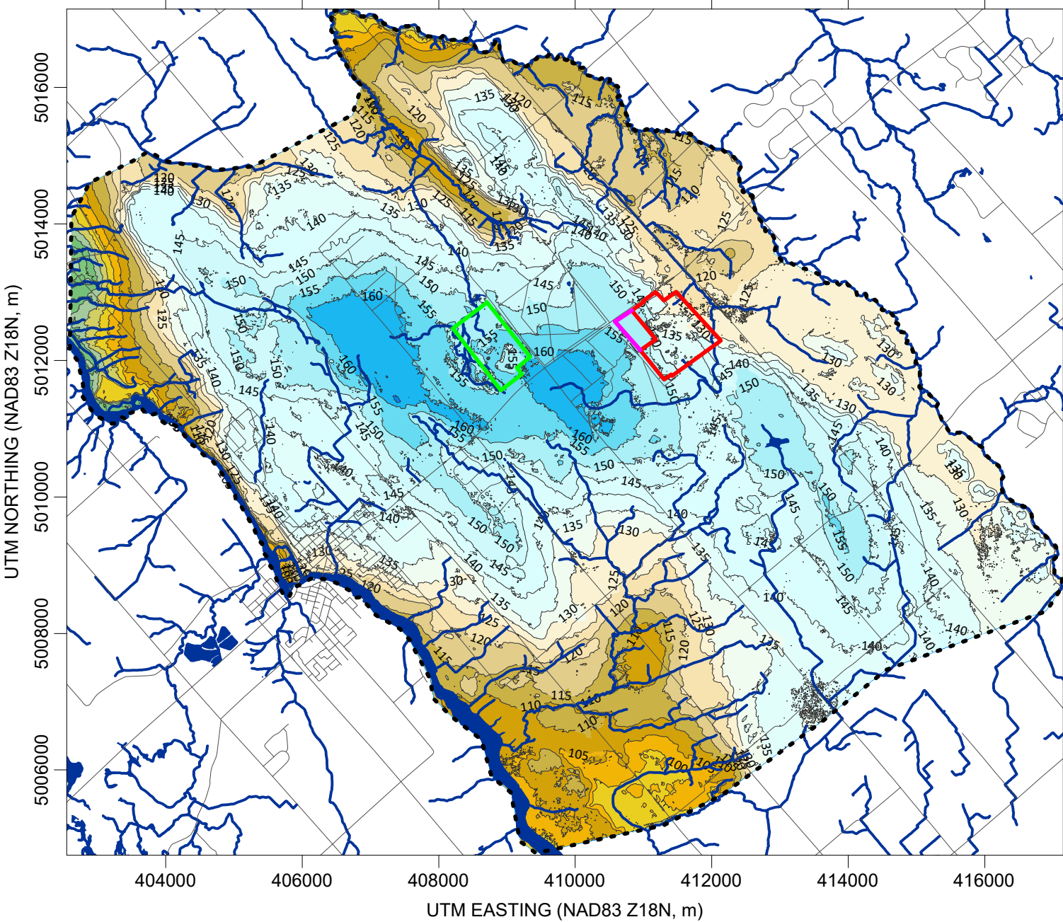
BEDROCK TOPOGRAPHY (masl)
