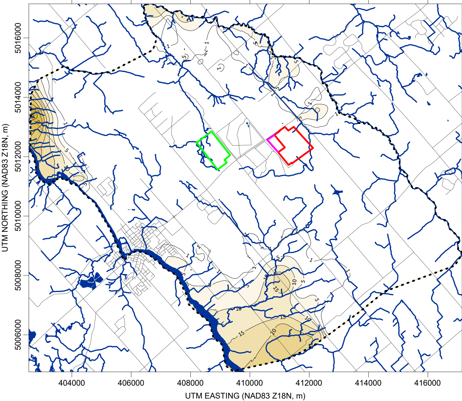
OVERBURDEN ISOPACH (m)
