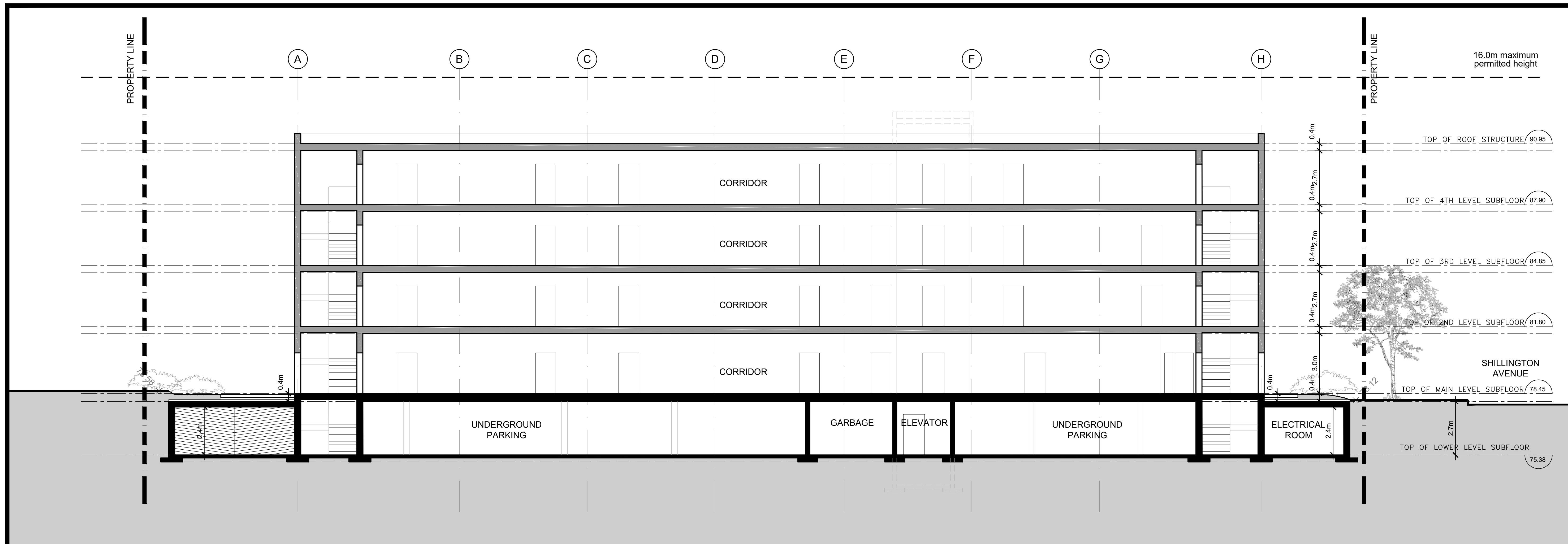
BUILDING SECTION
