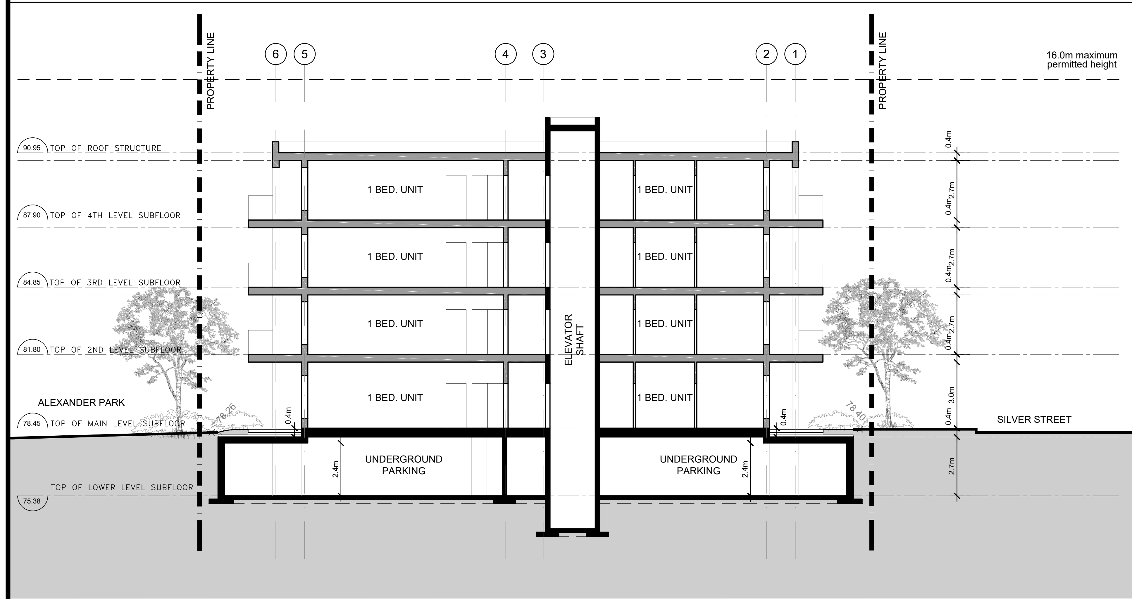
BUILDING SECTION
