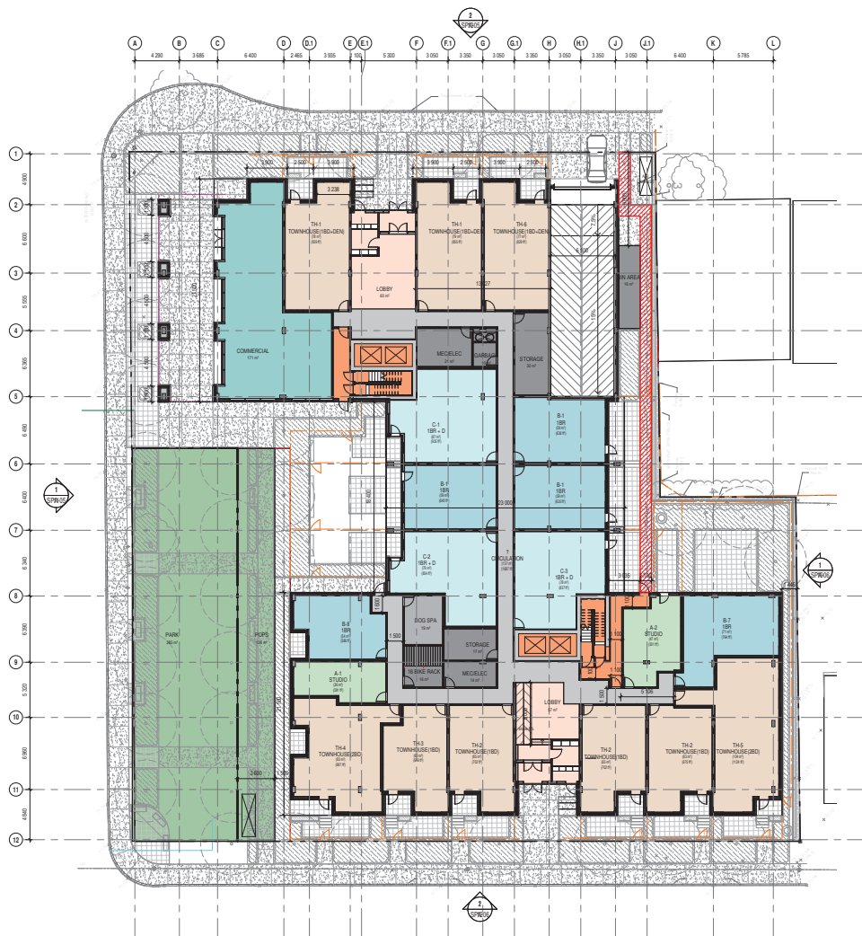
GROUND FLOOR 1:200
