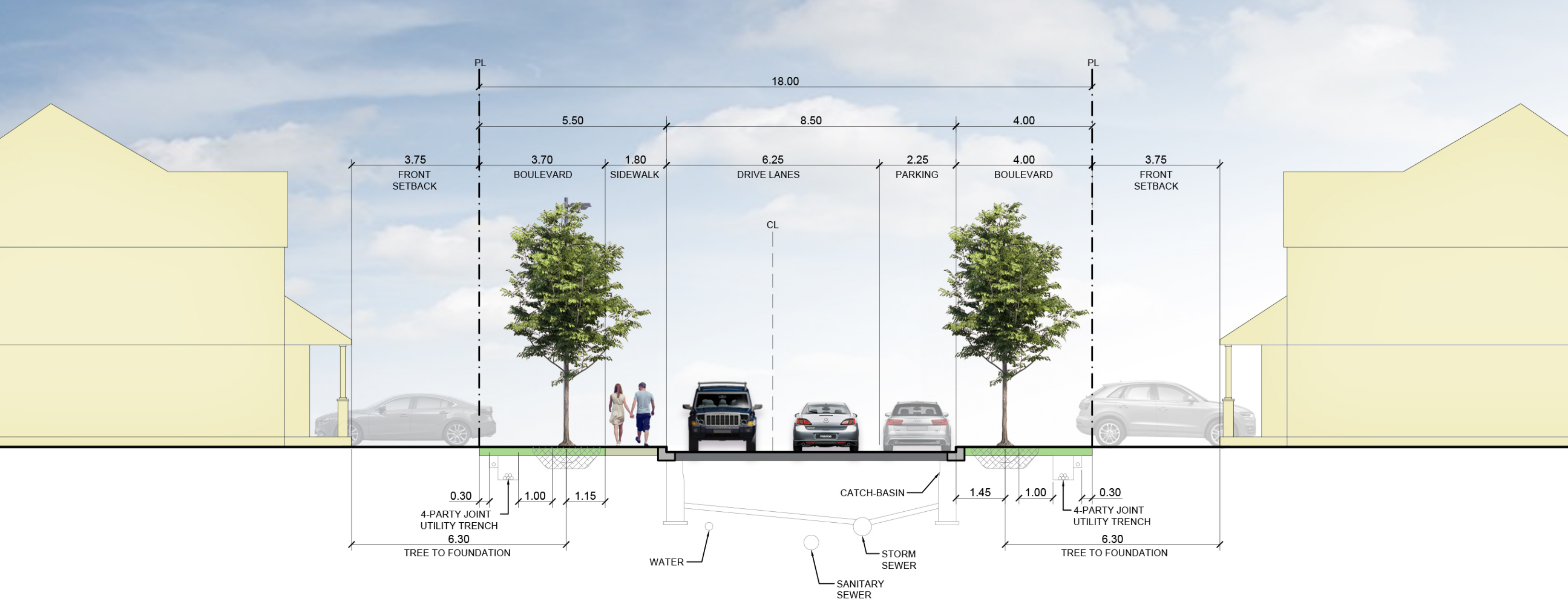
Figure 41 Local Road (Typical 18.0m Right-of-Way) Cross Section
