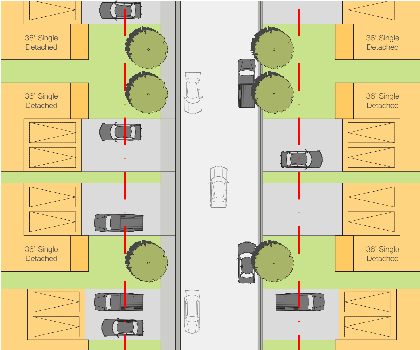
Figure 57 Single-Detached On-Street Parking Configuration
