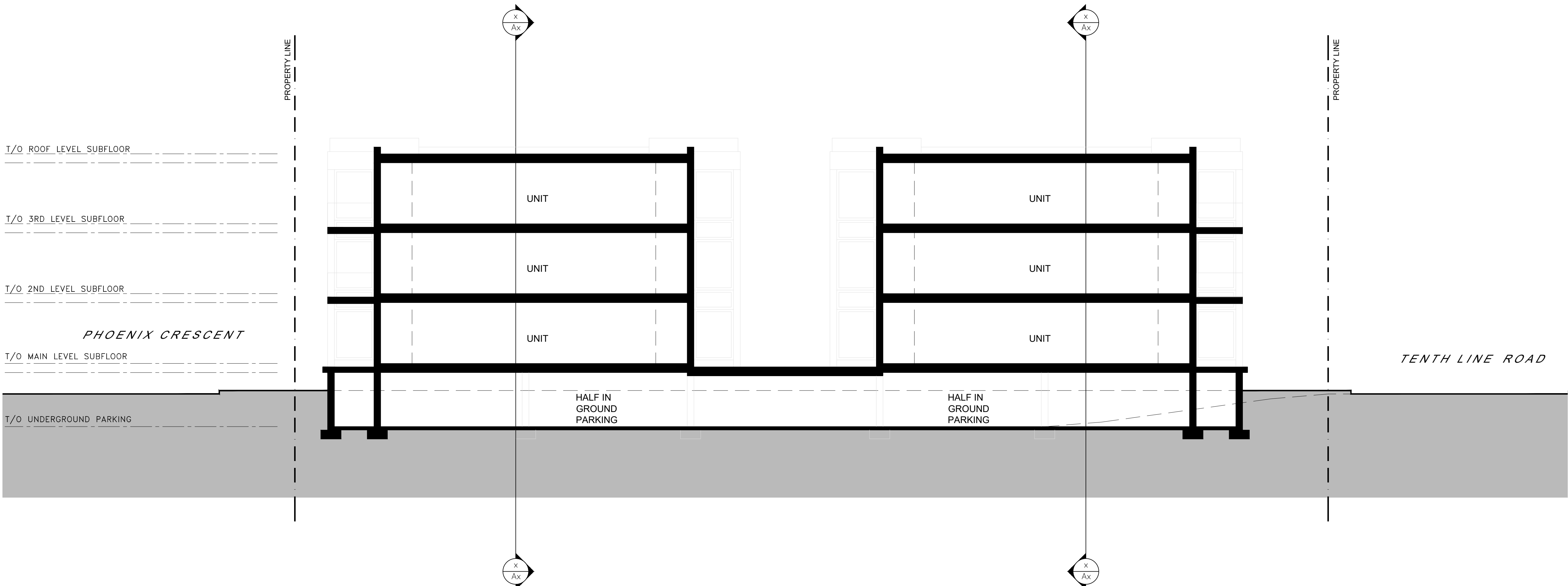
2 BUILDING SECTION SCALE = 1:100
